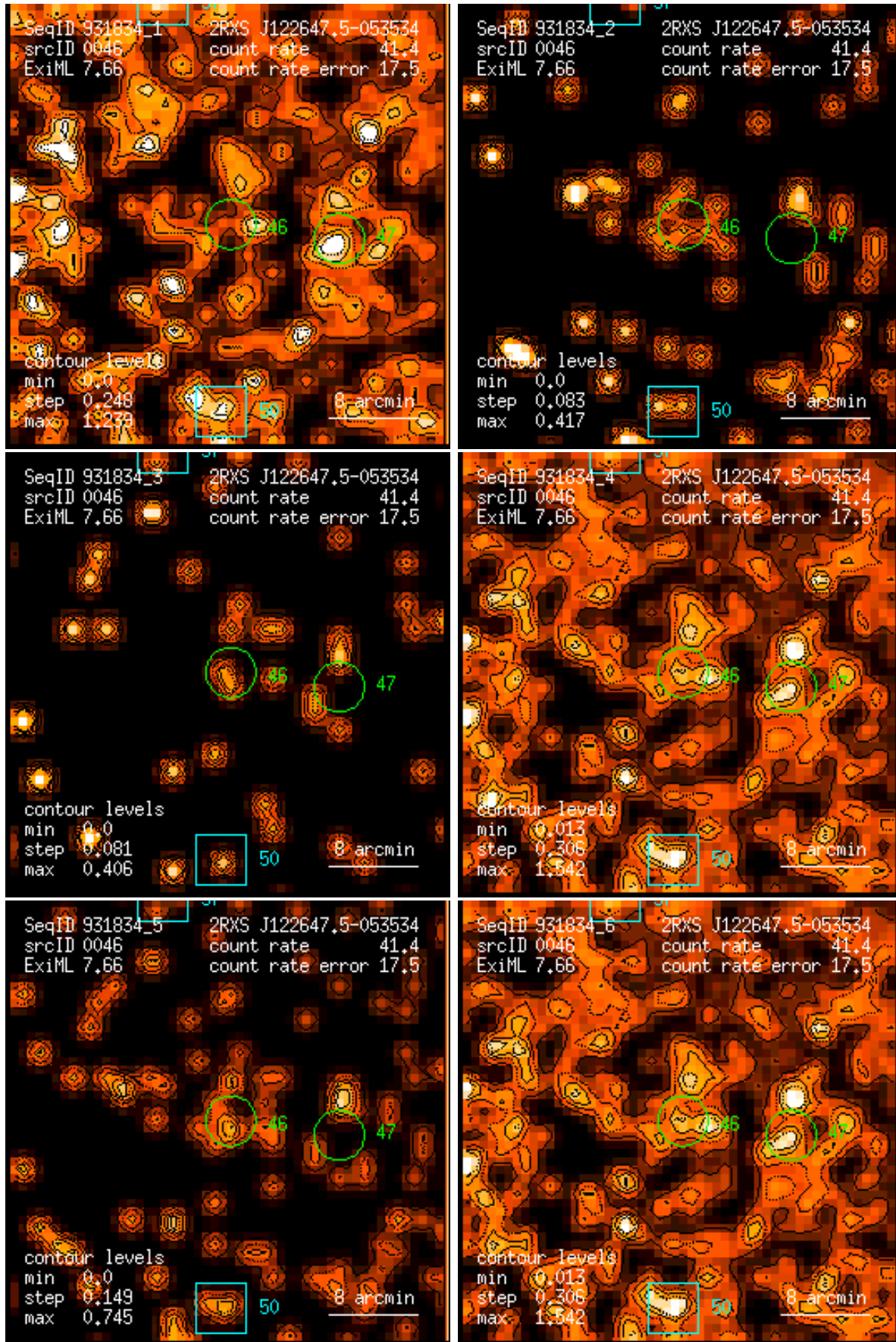
Figure 46: RASS 931834: detection 0046: band rate images, Gaussian filter: (1) PSPC channels 11 – 41, (2) 52 – 90, (3) 91 – 201, (4) 11 – 235, (5) 52 – 201, (6) 11 – 201. Broad band rates in counts/ks. Band rate contour levels in counts/ks/arcmin 2 .
