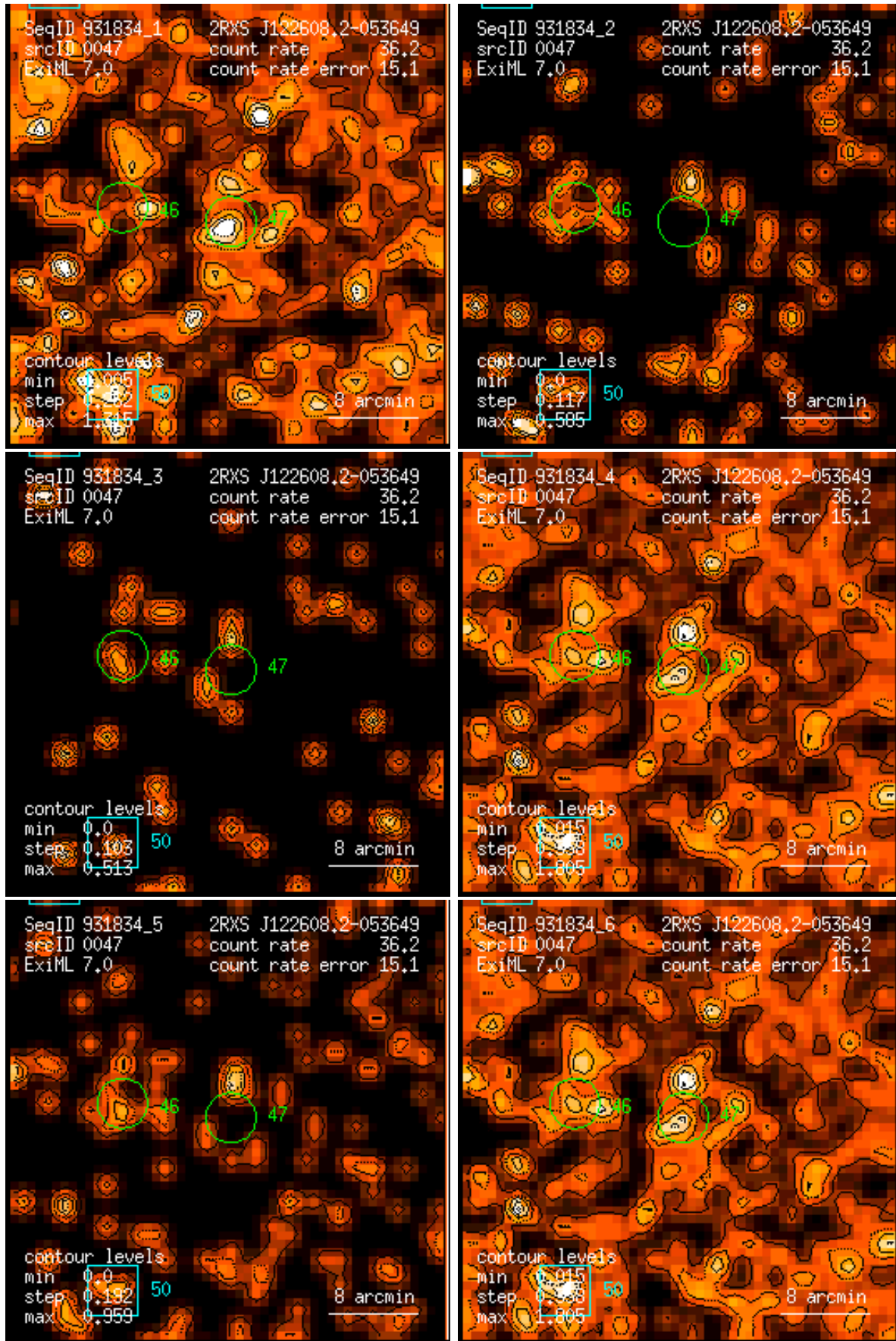
Figure 47: RASS 931834: detection 0047: band rate images, Gaussian filter: (1) PSPC channels 11 – 41, (2) 52 – 90, (3) 91 – 201, (4) 11 – 235, (5) 52 – 201, (6) 11 – 201. Broad band rates in counts/ks. Band rate contour levels in counts/ks/arcmin 2 .
