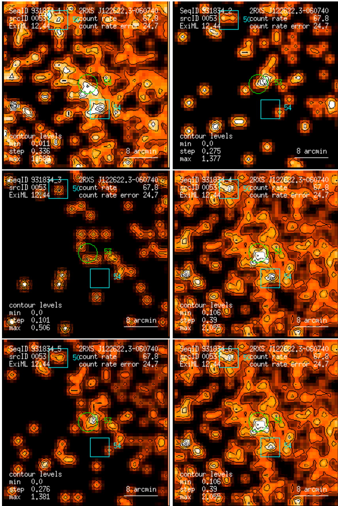
Figure 53: RASS 931834: detection 0053: band rate images, Gaussian filter: (1) PSPC channels 11 – 41, (2) 52 – 90, (3) 91 – 201, (4) 11 – 235, (5) 52 – 201, (6) 11 – 201. Broad band rates in counts/ks. Band rate contour levels in counts/ks/arcmin 2 .
