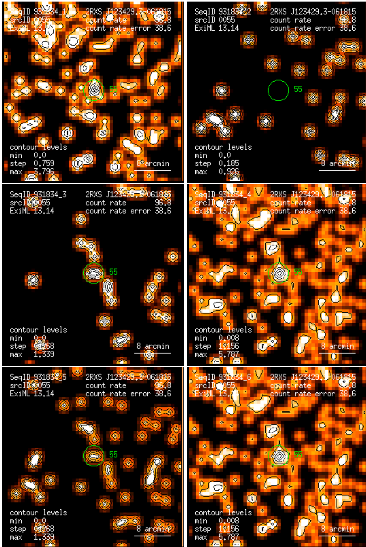
Figure 55: RASS 931834: detection 0055: band rate images, Gaussian filter: (1) PSPC channels 11 – 41, (2) 52 – 90, (3) 91 – 201, (4) 11 – 235, (5) 52 – 201, (6) 11 – 201. Broad band rates in counts/ks. Band rate contour levels in counts/ks/arcmin 2 .
