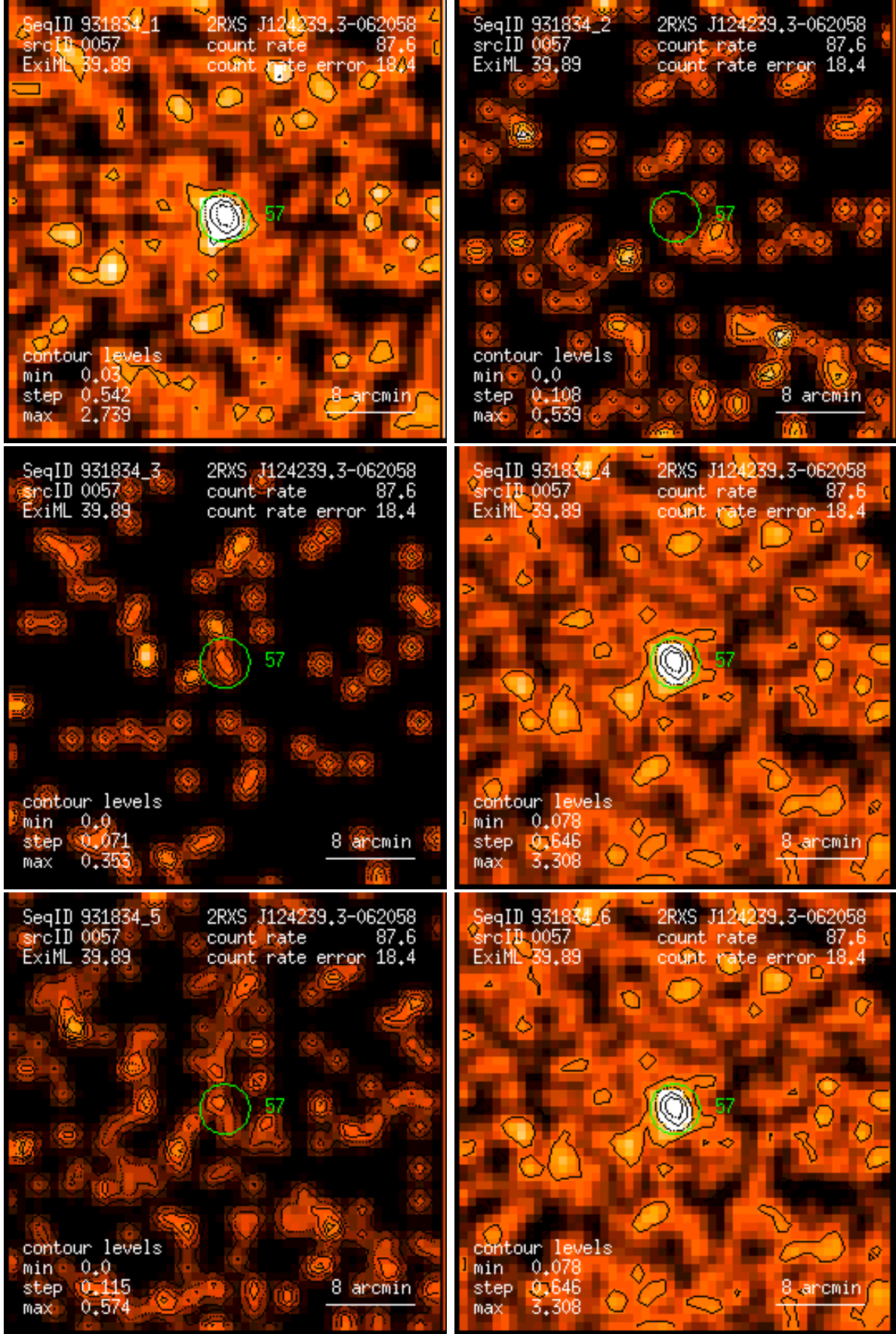
Figure 57: RASS 931834: detection 0057: band rate images, Gaussian filter: (1) PSPC channels 11 – 41, (2) 52 – 90, (3) 91 – 201, (4) 11 – 235, (5) 52 – 201, (6) 11 – 201. Broad band rates in counts/ks. Band rate contour levels in counts/ks/arcmin 2 .
