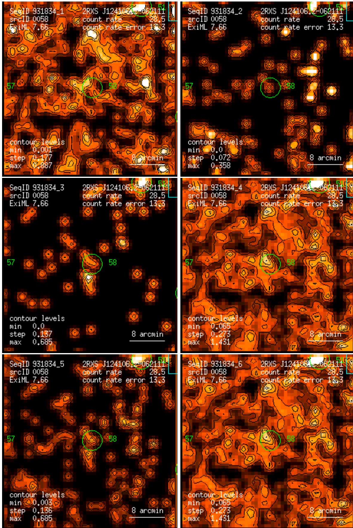
Figure 58: RASS 931834: detection 0058: band rate images, Gaussian filter: (1) PSPC channels 11 – 41, (2) 52 – 90, (3) 91 – 201, (4) 11 – 235, (5) 52 – 201, (6) 11 – 201. Broad band rates in counts/ks. Band rate contour levels in counts/ks/arcmin 2 .
