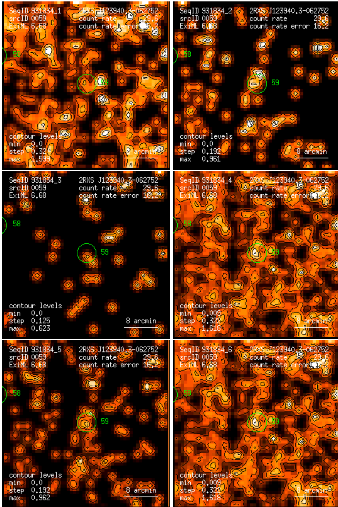
Figure 59: RASS 931834: detection 0059: band rate images, Gaussian filter: (1) PSPC channels 11 – 41, (2) 52 – 90, (3) 91 – 201, (4) 11 – 235, (5) 52 – 201, (6) 11 – 201. Broad band rates in counts/ks. Band rate contour levels in counts/ks/arcmin 2 .
