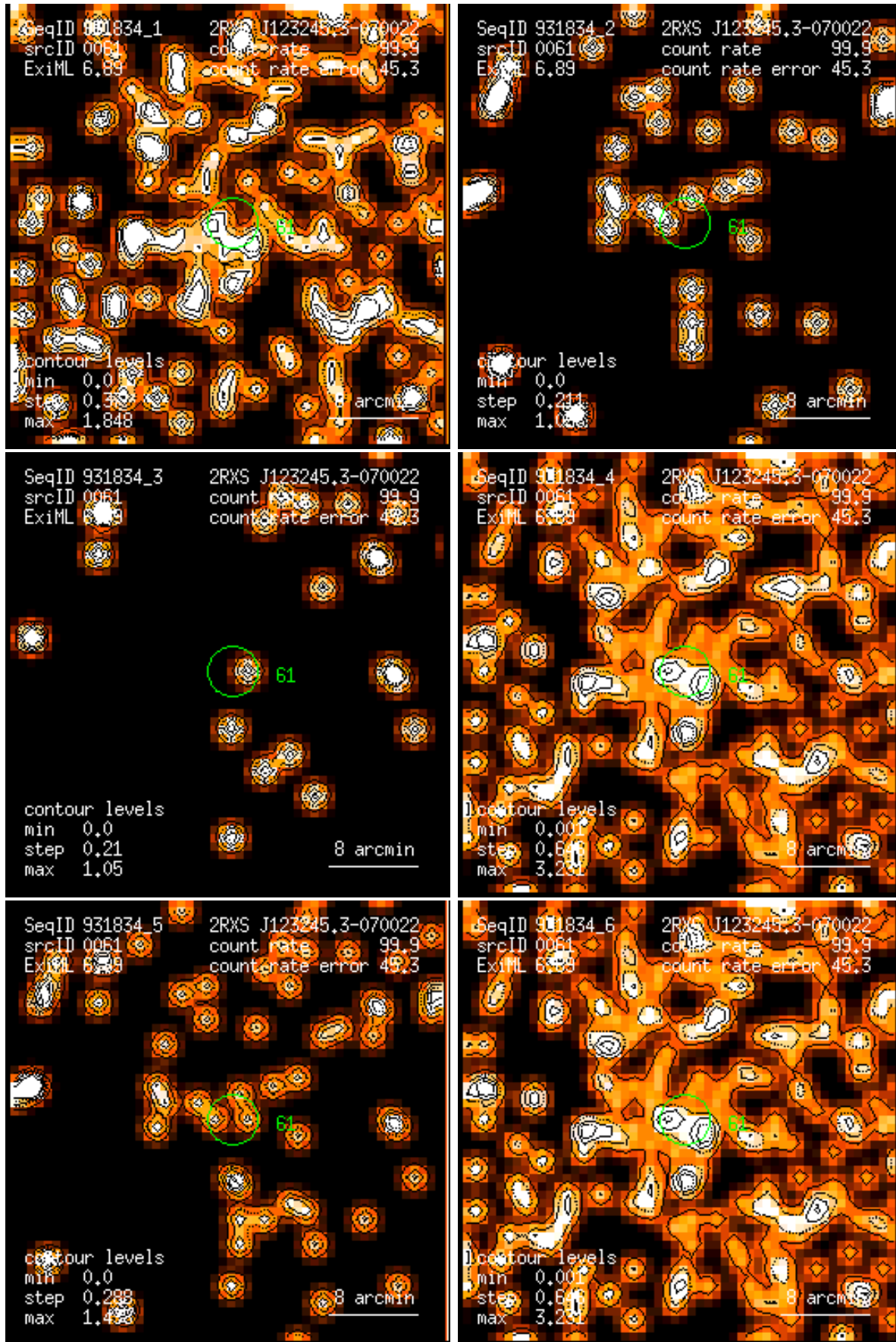
Figure 61: RASS 931834: detection 0061: band rate images, Gaussian filter: (1) PSPC channels 11 – 41, (2) 52 – 90, (3) 91 – 201, (4) 11 – 235, (5) 52 – 201, (6) 11 – 201. Broad band rates in counts/ks. Band rate contour levels in counts/ks/arcmin 2 .
