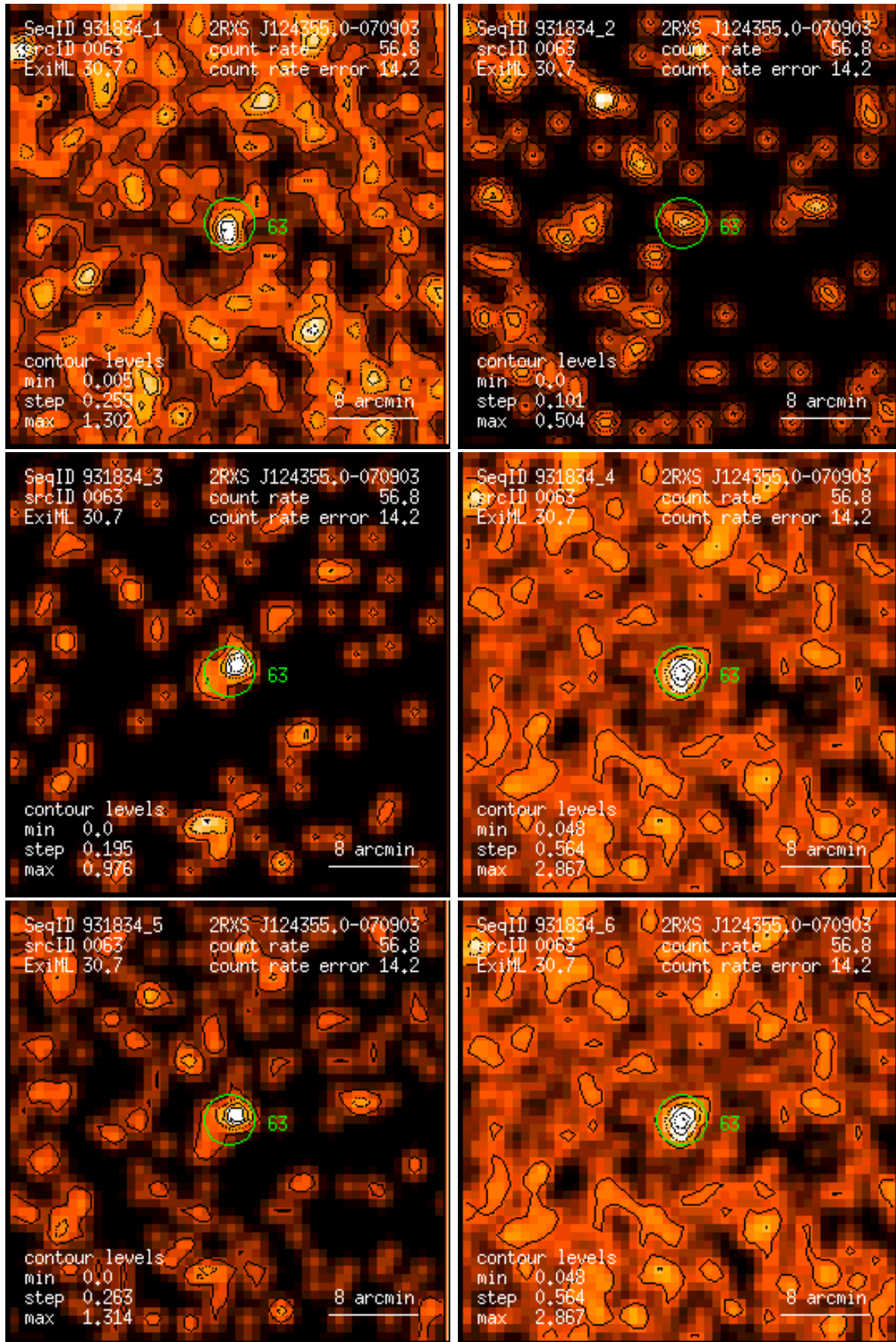
Figure 63: RASS 931834: detection 0063: band rate images, Gaussian filter: (1) PSPC channels 11 – 41, (2) 52 – 90, (3) 91 – 201, (4) 11 – 235, (5) 52 – 201, (6) 11 – 201. Broad band rates in counts/ks. Band rate contour levels in counts/ks/arcmin 2 .
