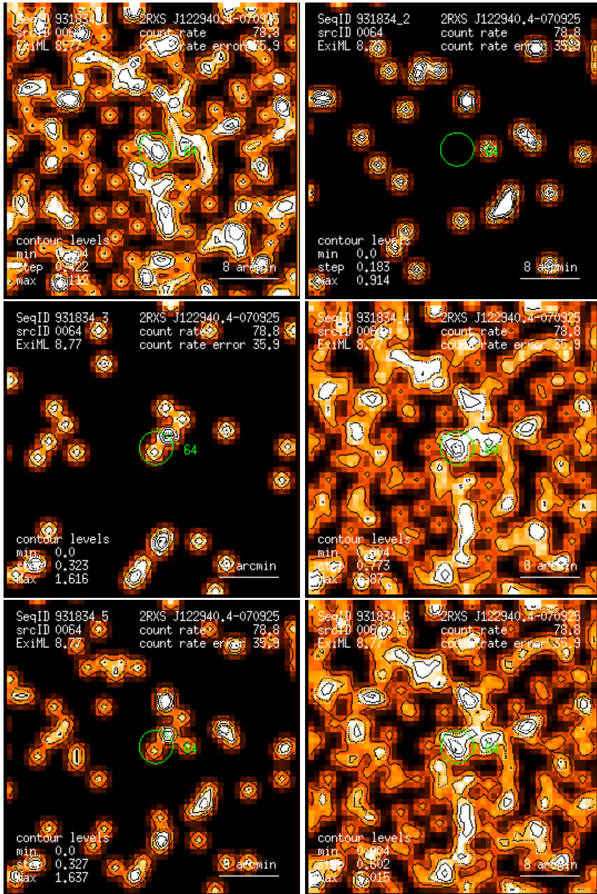
Figure 64: RASS 931834: detection 0064: band rate images, Gaussian filter: (1) PSPC channels 11 – 41, (2) 52 – 90, (3) 91 – 201, (4) 11 – 235, (5) 52 – 201, (6) 11 – 201. Broad band rates in counts/ks. Band rate contour levels in counts/ks/arcmin 2 .
