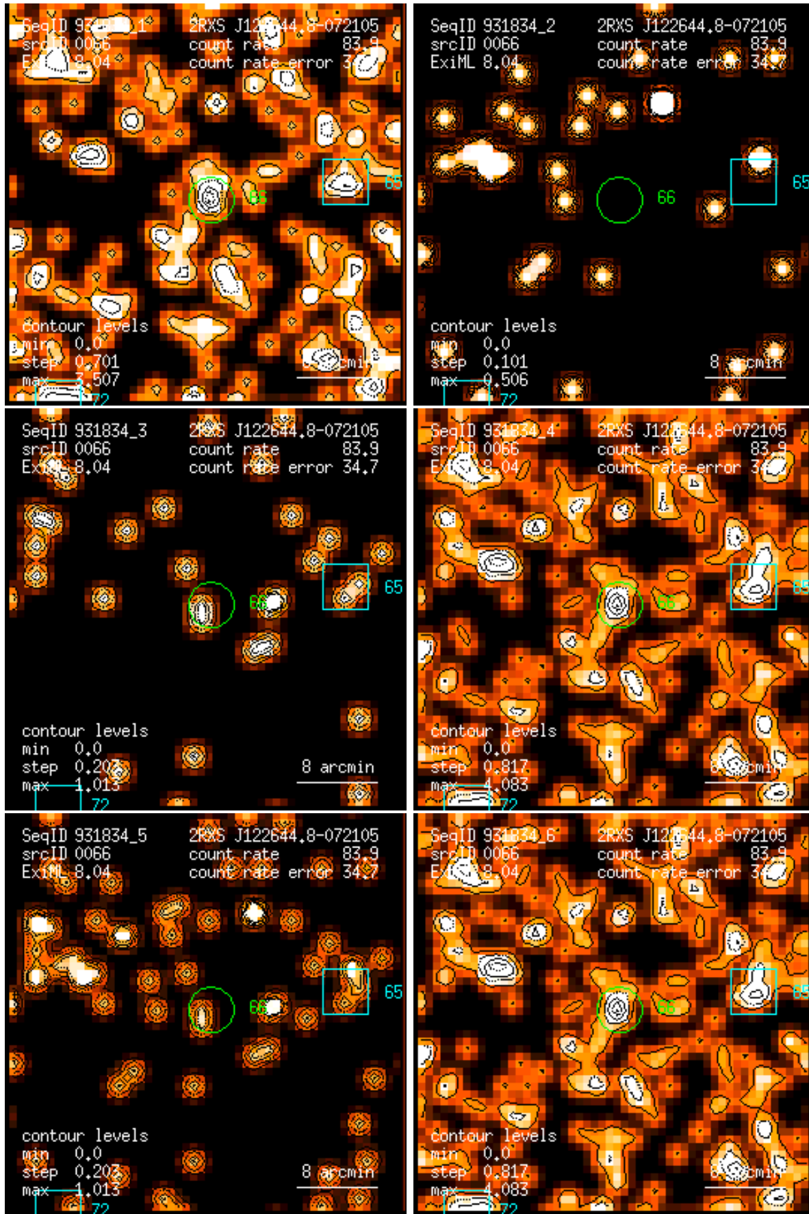
Figure 66: RASS 931834: detection 0066: band rate images, Gaussian filter: (1) PSPC channels 11 – 41, (2) 52 – 90, (3) 91 – 201, (4) 11 – 235, (5) 52 – 201, (6) 11 – 201. Broad band rates in counts/ks. Band rate contour levels in counts/ks/arcmin 2 .
