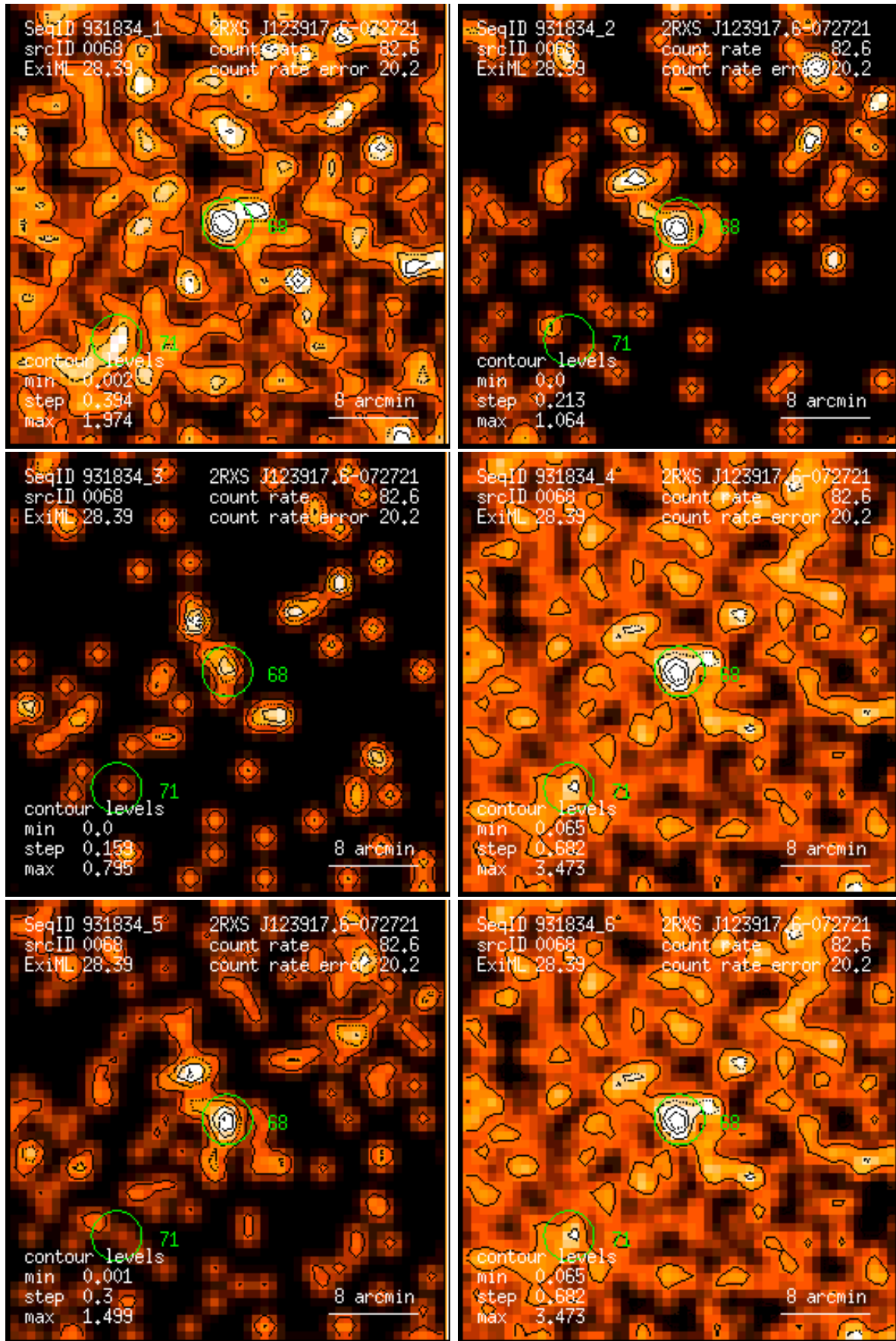
Figure 68: RASS 931834: detection 0068: band rate images, Gaussian filter: (1) PSPC channels 11 – 41, (2) 52 – 90, (3) 91 – 201, (4) 11 – 235, (5) 52 – 201, (6) 11 – 201. Broad band rates in counts/ks. Band rate contour levels in counts/ks/arcmin 2 .
