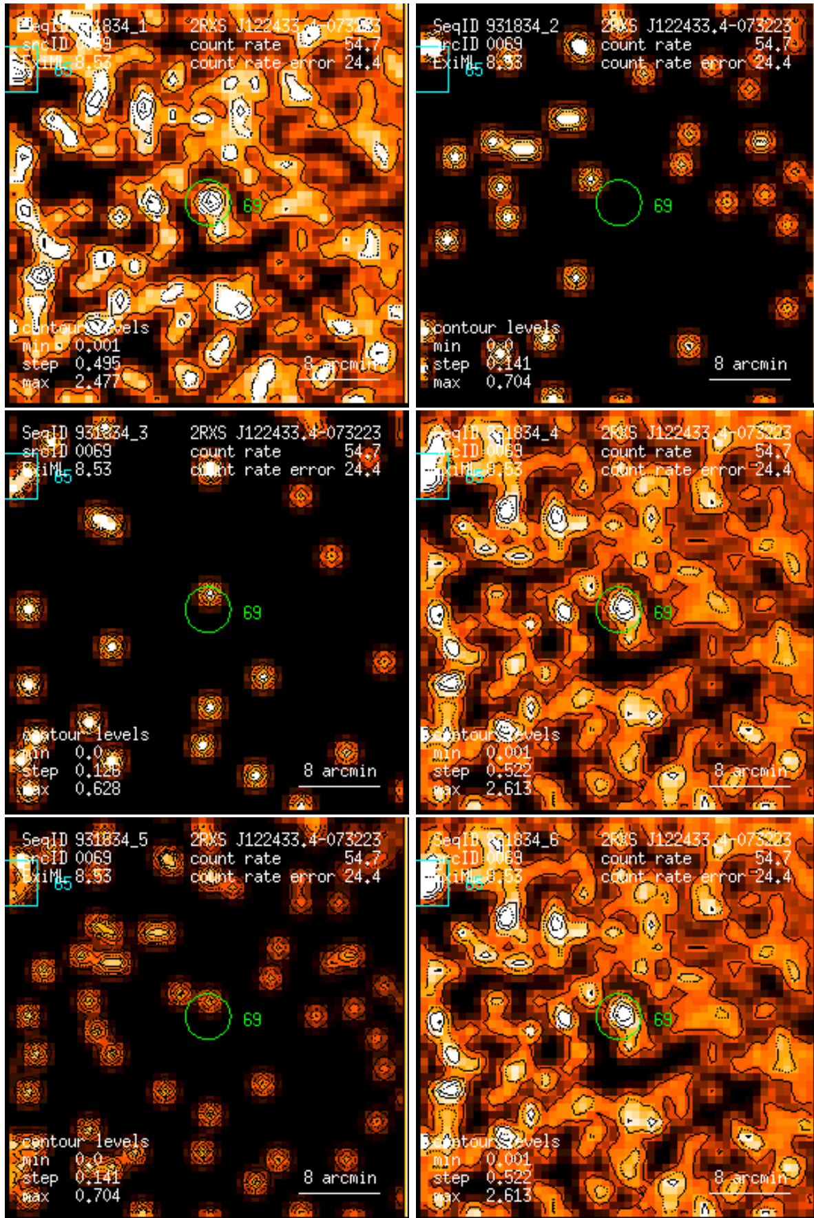
Figure 69: RASS 931834: detection 0069: band rate images, Gaussian filter: (1) PSPC channels 11 – 41, (2) 52 – 90, (3) 91 – 201, (4) 11 – 235, (5) 52 – 201, (6) 11 – 201. Broad band rates in counts/ks. Band rate contour levels in counts/ks/arcmin 2 .
