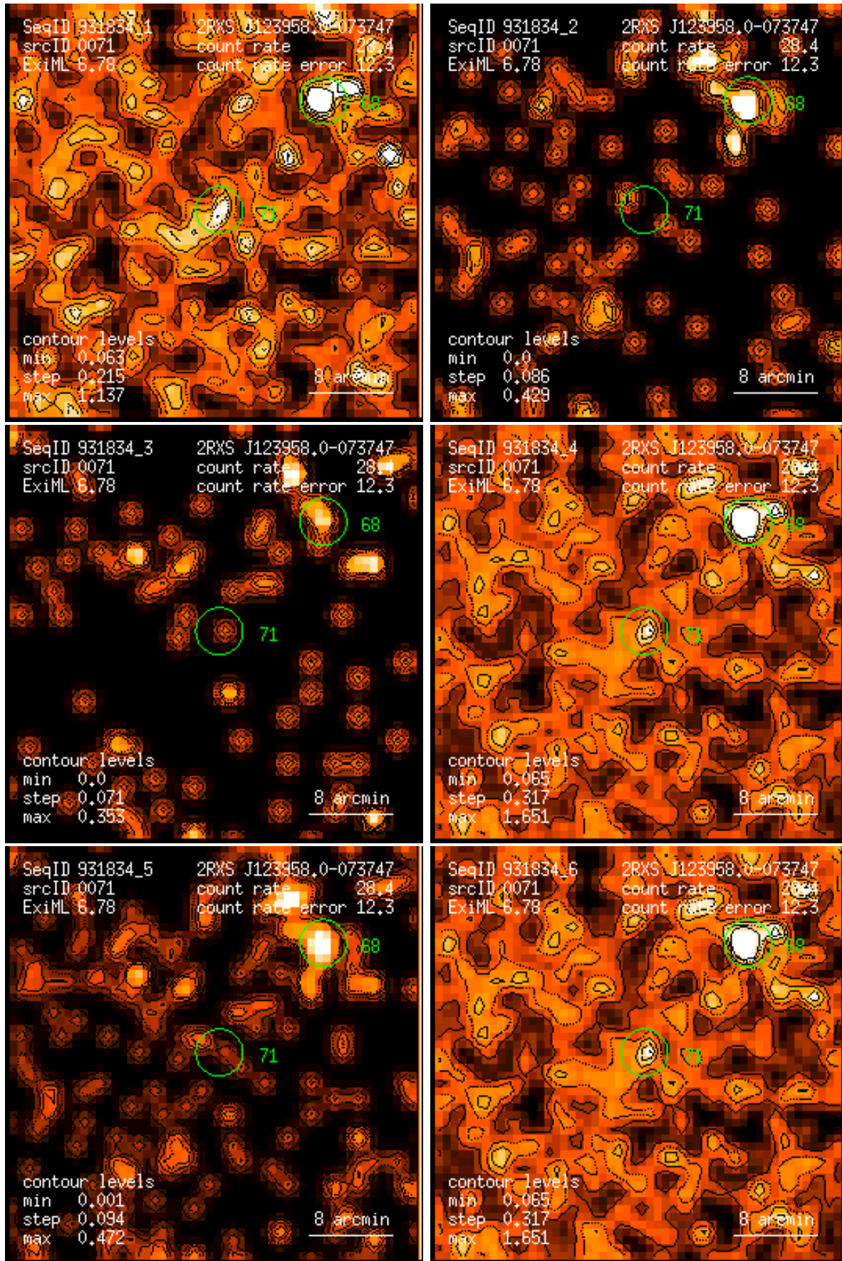
Figure 71: RASS 931834: detection 0071: band rate images, Gaussian filter: (1) PSPC channels 11 – 41, (2) 52 – 90, (3) 91 – 201, (4) 11 – 235, (5) 52 – 201, (6) 11 – 201. Broad band rates in counts/ks. Band rate contour levels in counts/ks/arcmin 2 .
