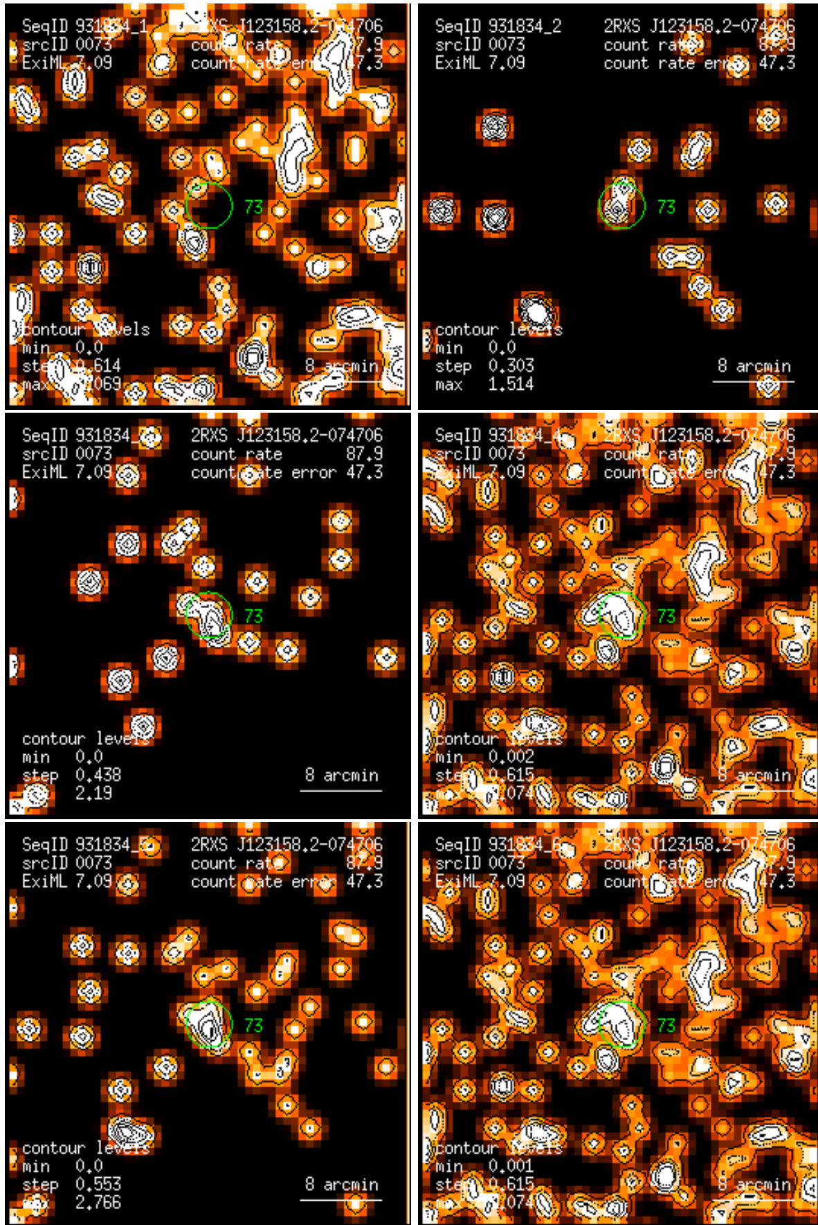
Figure 73: RASS 931834: detection 0073: band rate images, Gaussian filter: (1) PSPC channels 11 – 41, (2) 52 – 90, (3) 91 – 201, (4) 11 – 235, (5) 52 – 201, (6) 11 – 201. Broad band rates in counts/ks. Band rate contour levels in counts/ks/arcmin 2 .
