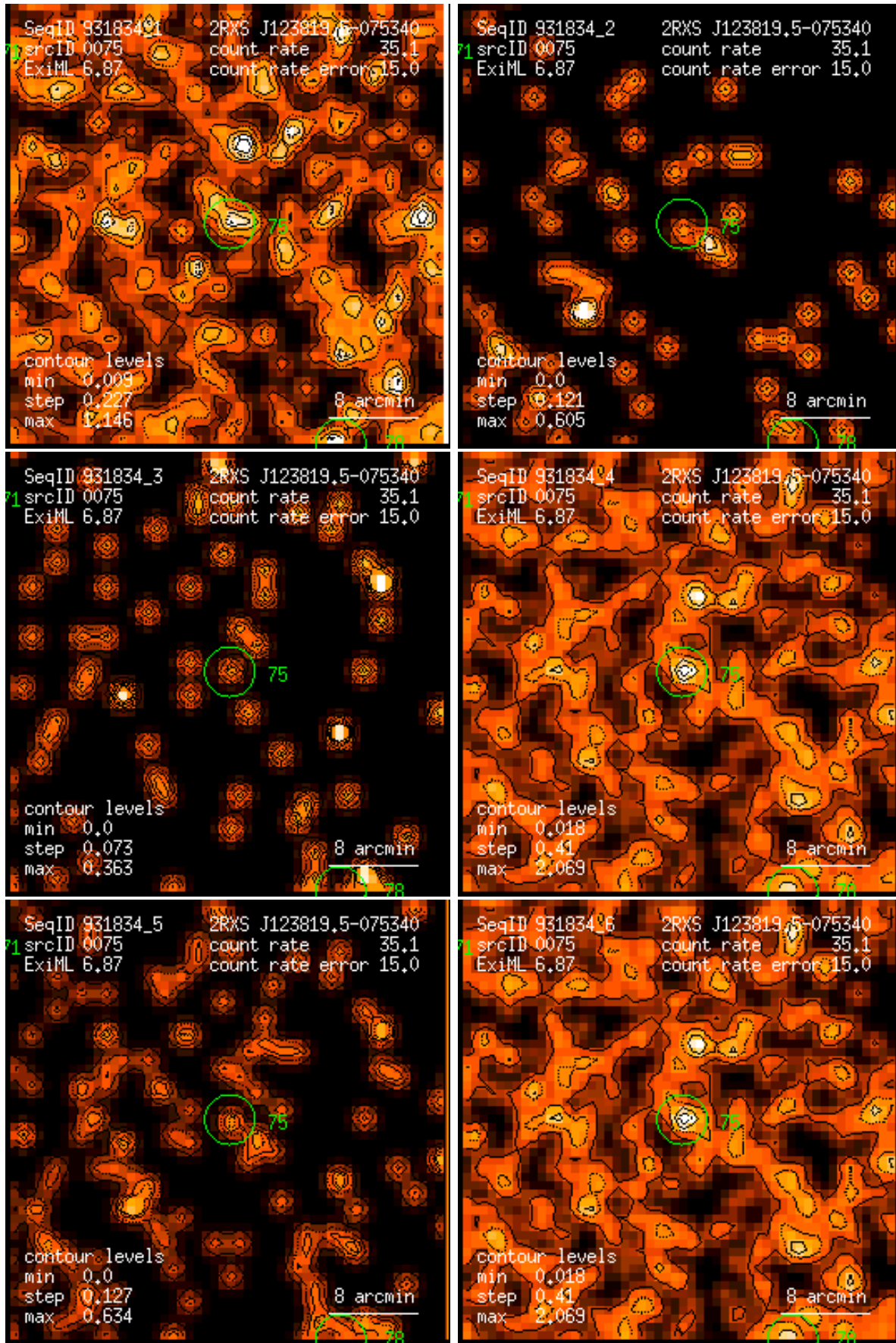
Figure 75: RASS 931834: detection 0075: band rate images, Gaussian filter: (1) PSPC channels 11 – 41, (2) 52 – 90, (3) 91 – 201, (4) 11 – 235, (5) 52 – 201, (6) 11 – 201. Broad band rates in counts/ks. Band rate contour levels in counts/ks/arcmin 2 .
