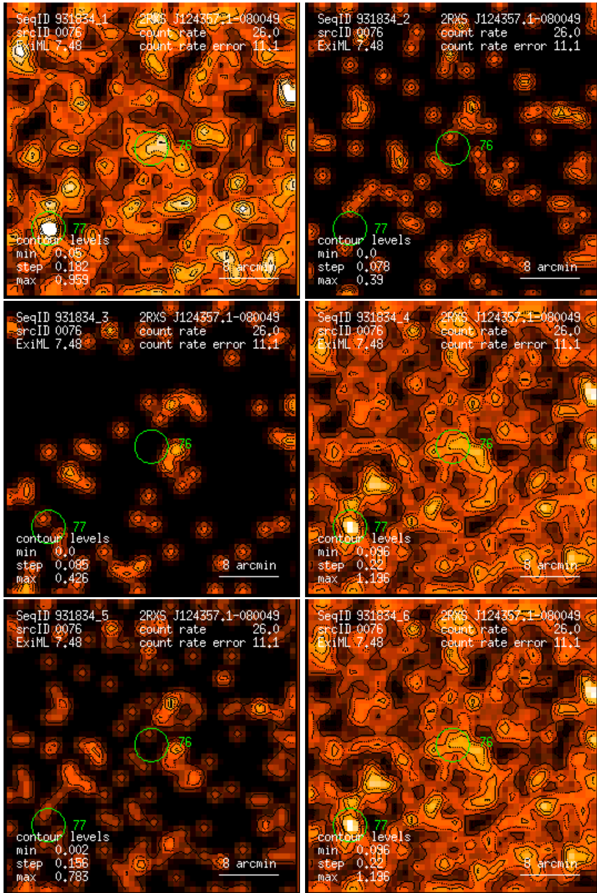
Figure 76: RASS 931834: detection 0076: band rate images, Gaussian filter: (1) PSPC channels 11 – 41, (2) 52 – 90, (3) 91 – 201, (4) 11 – 235, (5) 52 – 201, (6) 11 – 201. Broad band rates in counts/ks. Band rate contour levels in counts/ks/arcmin 2 .
