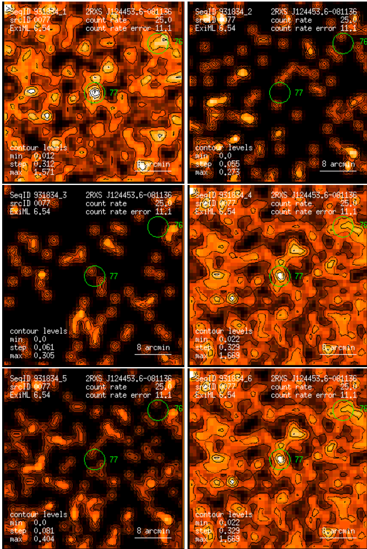
Figure 77: RASS 931834: detection 0077: band rate images, Gaussian filter: (1) PSPC channels 11 – 41, (2) 52 – 90, (3) 91 – 201, (4) 11 – 235, (5) 52 – 201, (6) 11 – 201. Broad band rates in counts/ks. Band rate contour levels in counts/ks/arcmin 2 .
