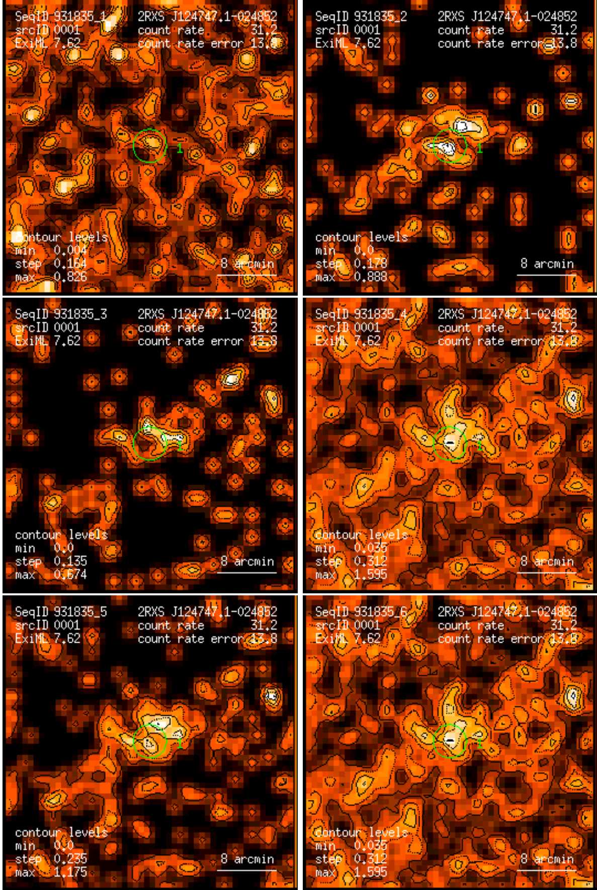
Figure 1: RASS 931835: detection 0001: band rate images, Gaussian filter: (1) PSPC channels 11 – 41, (2) 52 – 90, (3) 91 – 201, (4) 11 – 235, (5) 52 – 201, (6) 11 – 201. Broad band rates in counts/ks. Band rate contour levels in counts/ks/arcmin 2 .
