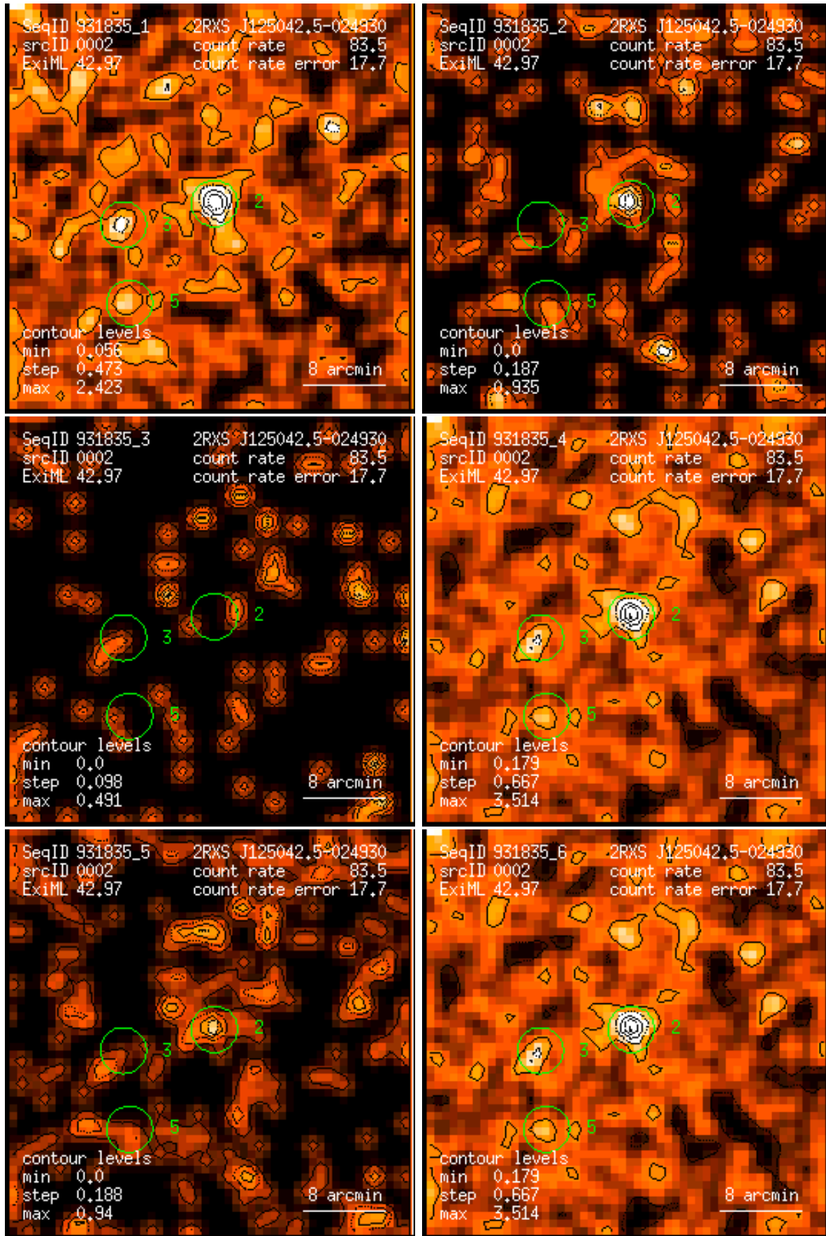
Figure 2: RASS 931835: detection 0002: band rate images, Gaussian filter: (1) PSPC channels 11 – 41, (2) 52 – 90, (3) 91 – 201, (4) 11 – 235, (5) 52 – 201, (6) 11 – 201. Broad band rates in counts/ks. Band rate contour levels in counts/ks/arcmin 2 .
