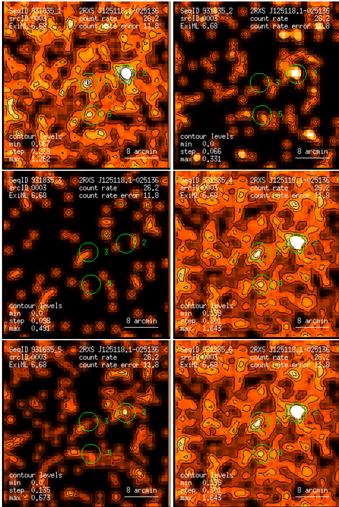
Figure 3: RASS 931835: detection 0003: band rate images, Gaussian filter: (1) PSPC channels 11 – 41, (2) 52 – 90, (3) 91 – 201, (4) 11 – 235, (5) 52 – 201, (6) 11 – 201. Broad band rates in counts/ks. Band rate contour levels in counts/ks/arcmin 2 .
