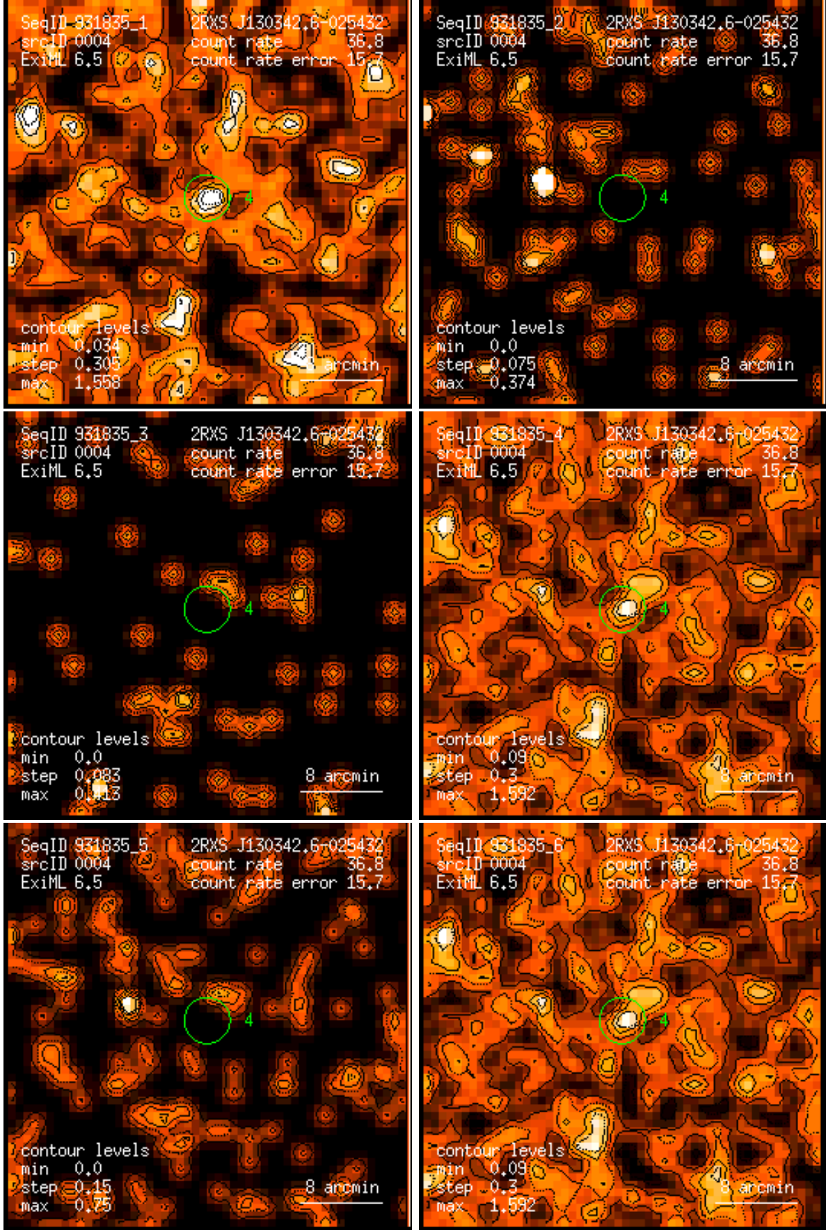
Figure 4: RASS 931835: detection 0004: band rate images, Gaussian filter: (1) PSPC channels 11 – 41, (2) 52 – 90, (3) 91 – 201, (4) 11 – 235, (5) 52 – 201, (6) 11 – 201. Broad band rates in counts/ks. Band rate contour levels in counts/ks/arcmin 2 .
