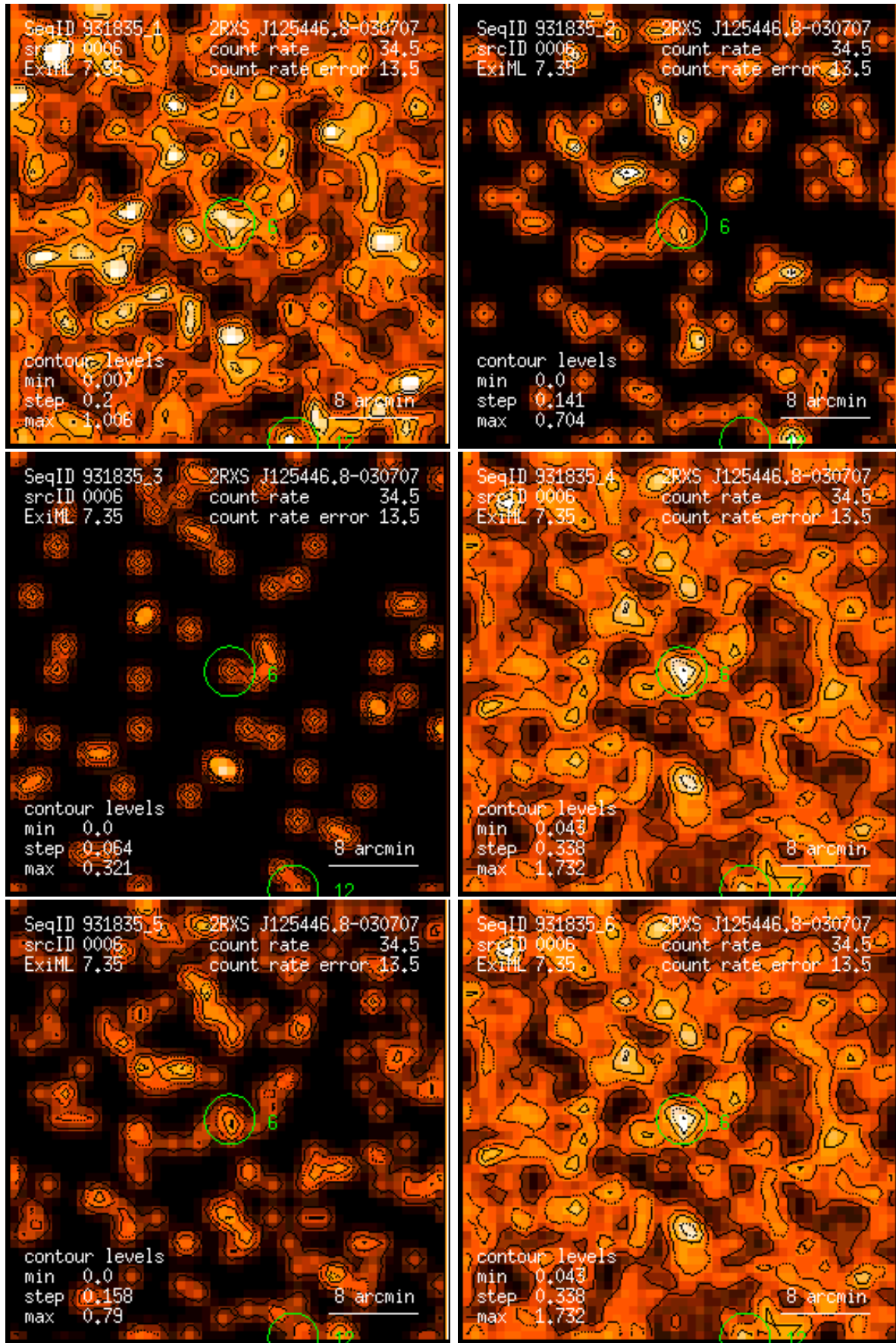
Figure 6: RASS 931835: detection 0006: band rate images, Gaussian filter: (1) PSPC channels 11 – 41, (2) 52 – 90, (3) 91 – 201, (4) 11 – 235, (5) 52 – 201, (6) 11 – 201. Broad band rates in counts/ks. Band rate contour levels in counts/ks/arcmin 2 .
