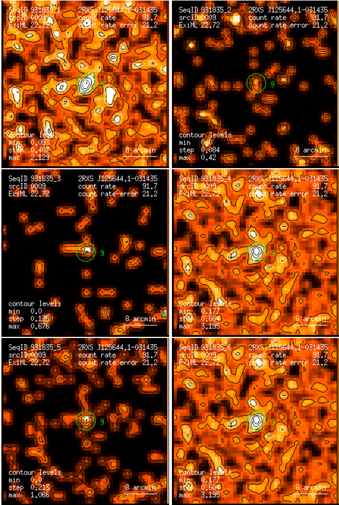
Figure 9: RASS 931835: detection 0009: band rate images, Gaussian filter: (1) PSPC channels 11 – 41, (2) 52 – 90, (3) 91 – 201, (4) 11 – 235, (5) 52 – 201, (6) 11 – 201. Broad band rates in counts/ks. Band rate contour levels in counts/ks/arcmin 2 .
