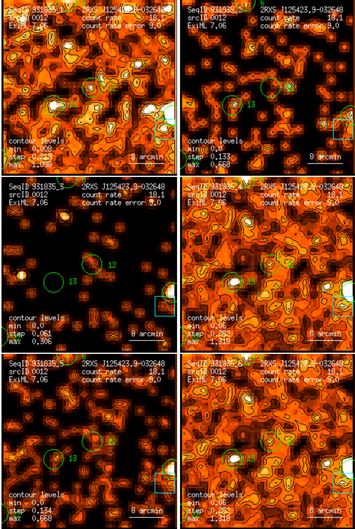
Figure 12: RASS 931835: detection 0012: band rate images, Gaussian filter: (1) PSPC channels 11 – 41, (2) 52 – 90, (3) 91 – 201, (4) 11 – 235, (5) 52 – 201, (6) 11 – 201. Broad band rates in counts/ks. Band rate contour levels in counts/ks/arcmin 2 .
