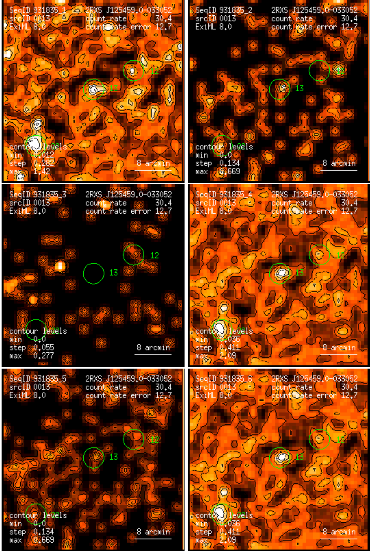
Figure 13: RASS 931835: detection 0013: band rate images, Gaussian filter: (1) PSPC channels 11 – 41, (2) 52 – 90, (3) 91 – 201, (4) 11 – 235, (5) 52 – 201, (6) 11 – 201. Broad band rates in counts/ks. Band rate contour levels in counts/ks/arcmin 2 .
