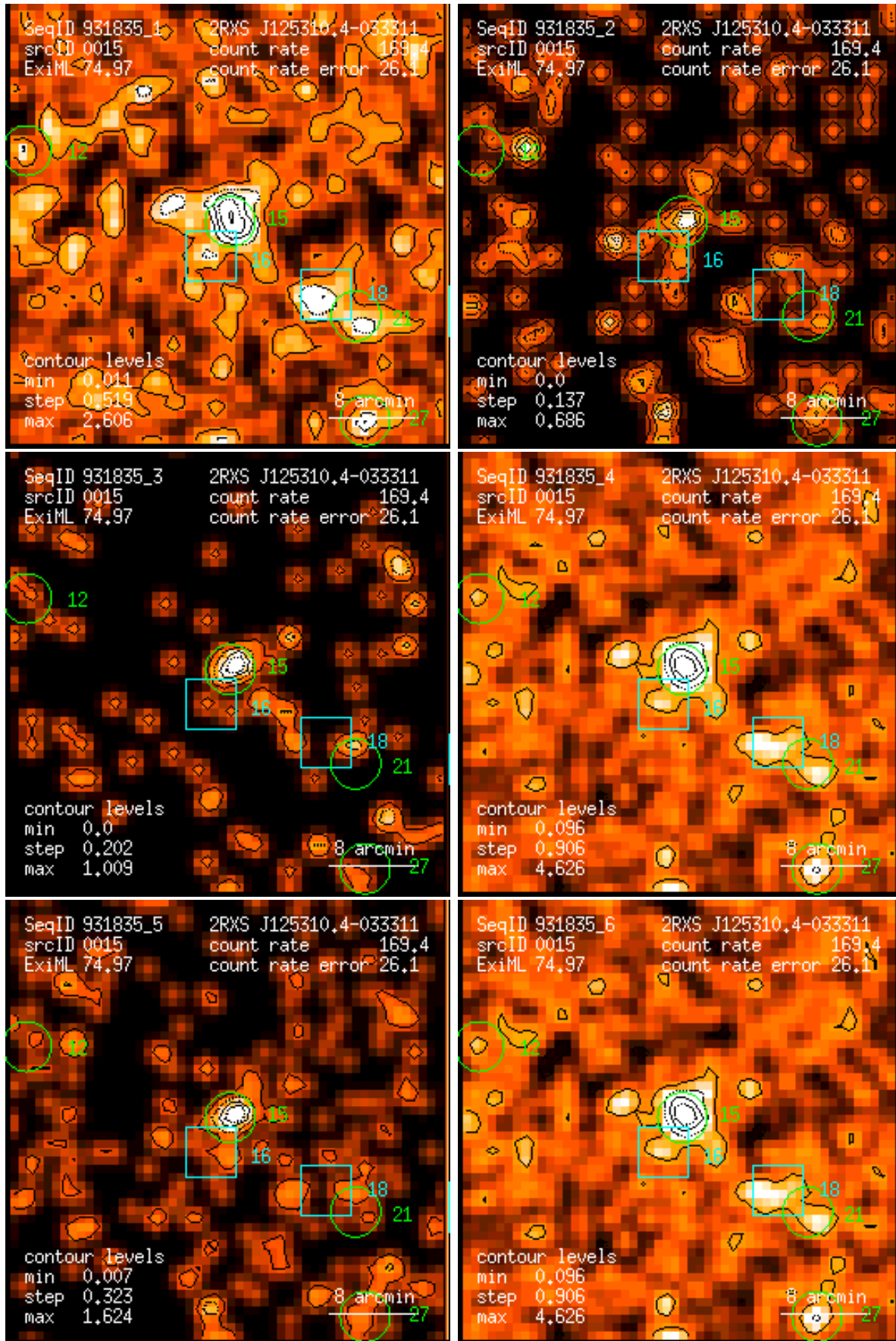
Figure 15: RASS 931835: detection 0015: band rate images, Gaussian filter: (1) PSPC channels 11 – 41, (2) 52 – 90, (3) 91 – 201, (4) 11 – 235, (5) 52 – 201, (6) 11 – 201. Broad band rates in counts/ks. Band rate contour levels in counts/ks/arcmin 2 .
