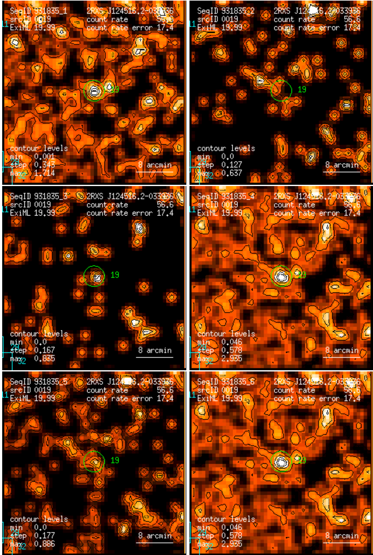
Figure 19: RASS 931835: detection 0019: band rate images, Gaussian filter: (1) PSPC channels 11 – 41, (2) 52 – 90, (3) 91 – 201, (4) 11 – 235, (5) 52 – 201, (6) 11 – 201. Broad band rates in counts/ks. Band rate contour levels in counts/ks/arcmin 2 .
