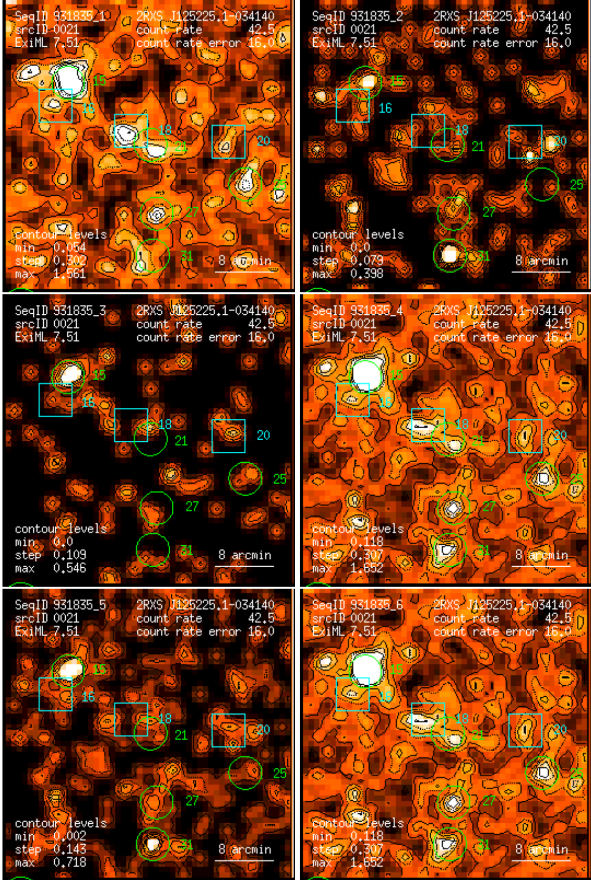
Figure 21: RASS 931835: detection 0021: band rate images, Gaussian filter: (1) PSPC channels 11 – 41, (2) 52 – 90, (3) 91 – 201, (4) 11 – 235, (5) 52 – 201, (6) 11 – 201. Broad band rates in counts/ks. Band rate contour levels in counts/ks/arcmin 2 .
