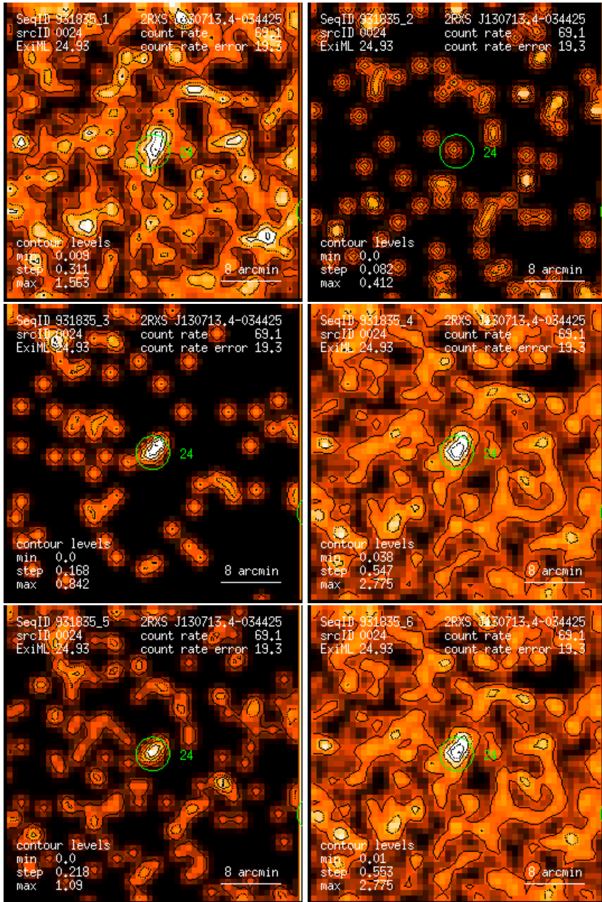
Figure 24: RASS 931835: detection 0024: band rate images, Gaussian filter: (1) PSPC channels 11 – 41, (2) 52 – 90, (3) 91 – 201, (4) 11 – 235, (5) 52 – 201, (6) 11 – 201. Broad band rates in counts/ks. Band rate contour levels in counts/ks/arcmin 2 .
