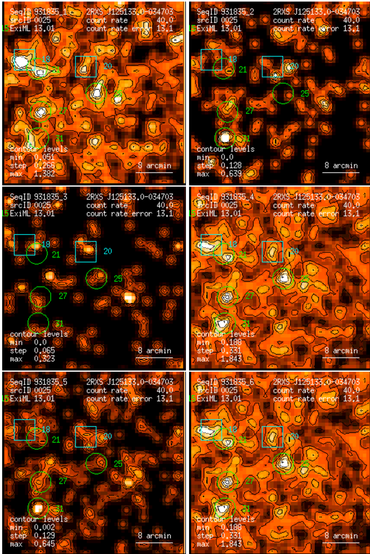
Figure 25: RASS 931835: detection 0025: band rate images, Gaussian filter: (1) PSPC channels 11 – 41, (2) 52 – 90, (3) 91 – 201, (4) 11 – 235, (5) 52 – 201, (6) 11 – 201. Broad band rates in counts/ks. Band rate contour levels in counts/ks/arcmin 2 .
