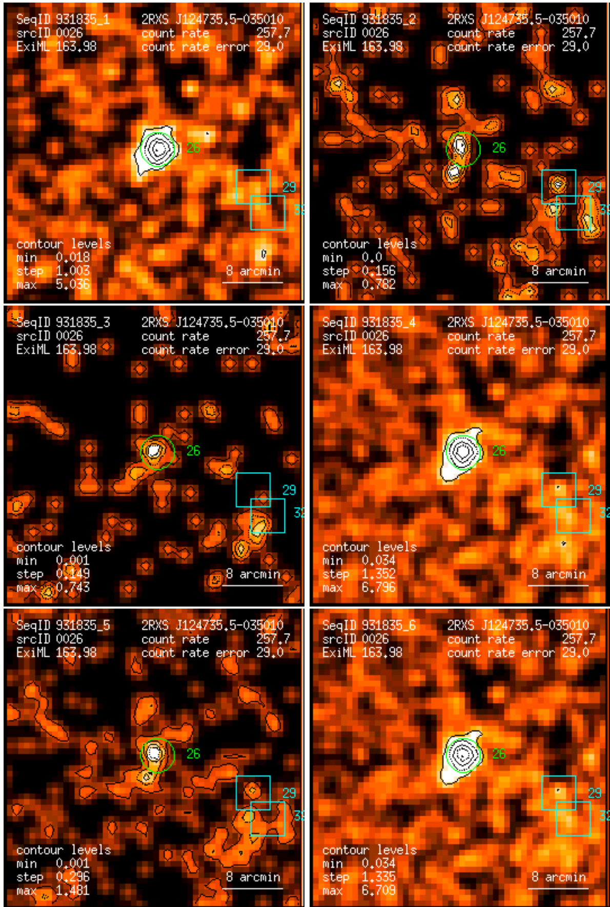
Figure 26: RASS 931835: detection 0026: band rate images, Gaussian filter: (1) PSPC channels 11 – 41, (2) 52 – 90, (3) 91 – 201, (4) 11 – 235, (5) 52 – 201, (6) 11 – 201. Broad band rates in counts/ks. Band rate contour levels in counts/ks/arcmin 2 .
