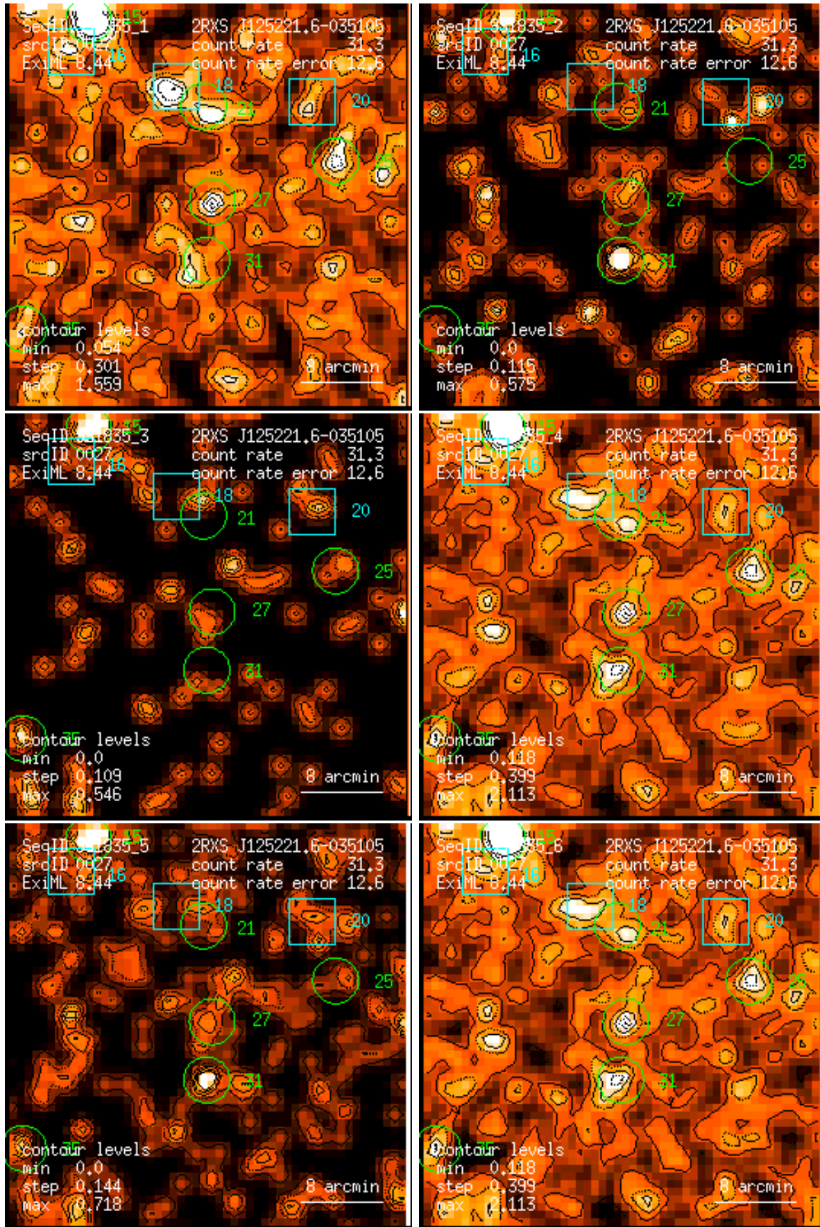
Figure 27: RASS 931835: detection 0027: band rate images, Gaussian filter: (1) PSPC channels 11 – 41, (2) 52 – 90, (3) 91 – 201, (4) 11 – 235, (5) 52 – 201, (6) 11 – 201. Broad band rates in counts/ks. Band rate contour levels in counts/ks/arcmin 2 .
