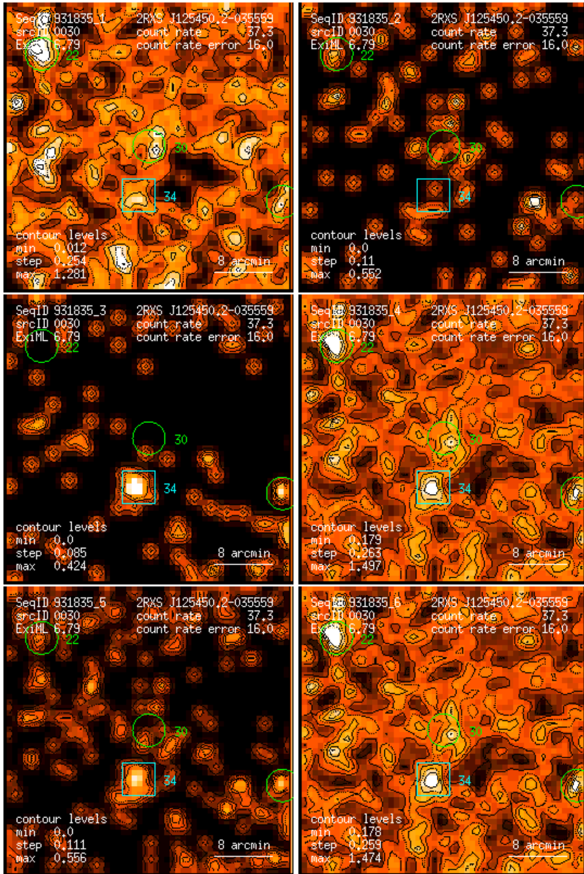
Figure 30: RASS 931835: detection 0030: band rate images, Gaussian filter: (1) PSPC channels 11 – 41, (2) 52 – 90, (3) 91 – 201, (4) 11 – 235, (5) 52 – 201, (6) 11 – 201. Broad band rates in counts/ks. Band rate contour levels in counts/ks/arcmin 2 .
