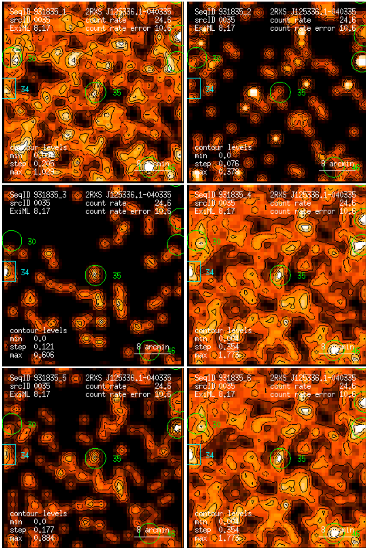
Figure 35: RASS 931835: detection 0035: band rate images, Gaussian filter: (1) PSPC channels 11 – 41, (2) 52 – 90, (3) 91 – 201, (4) 11 – 235, (5) 52 – 201, (6) 11 – 201. Broad band rates in counts/ks. Band rate contour levels in counts/ks/arcmin 2 .
