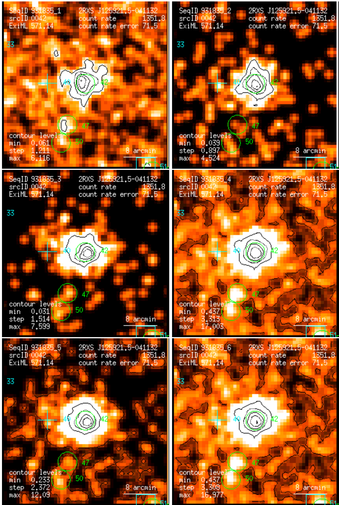
Figure 42: RASS 931835: detection 0042: band rate images, Gaussian filter: (1) PSPC channels 11 – 41, (2) 52 – 90, (3) 91 – 201, (4) 11 – 235, (5) 52 – 201, (6) 11 – 201. Broad band rates in counts/ks. Band rate contour levels in counts/ks/arcmin 2 .
