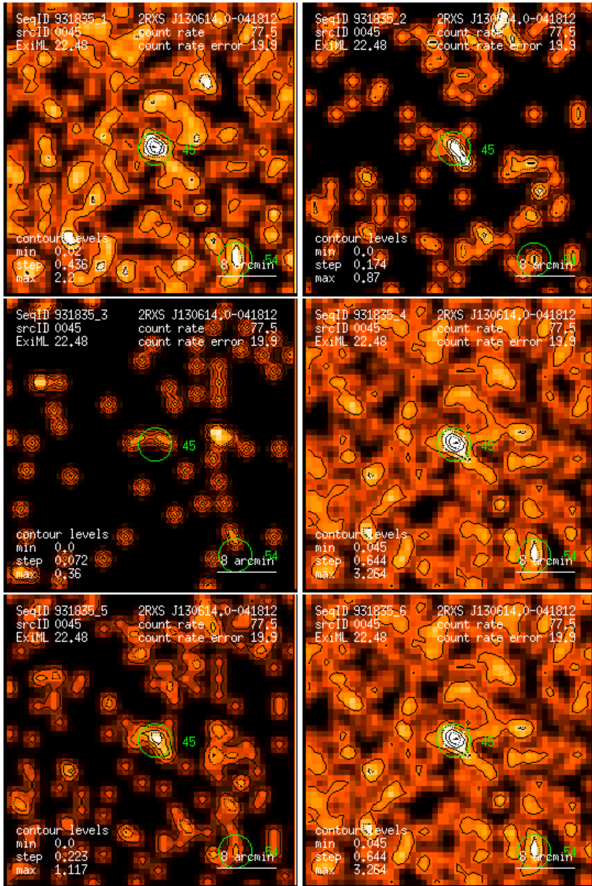
Figure 45: RASS 931835: detection 0045: band rate images, Gaussian filter: (1) PSPC channels 11 – 41, (2) 52 – 90, (3) 91 – 201, (4) 11 – 235, (5) 52 – 201, (6) 11 – 201. Broad band rates in counts/ks. Band rate contour levels in counts/ks/arcmin 2 .
