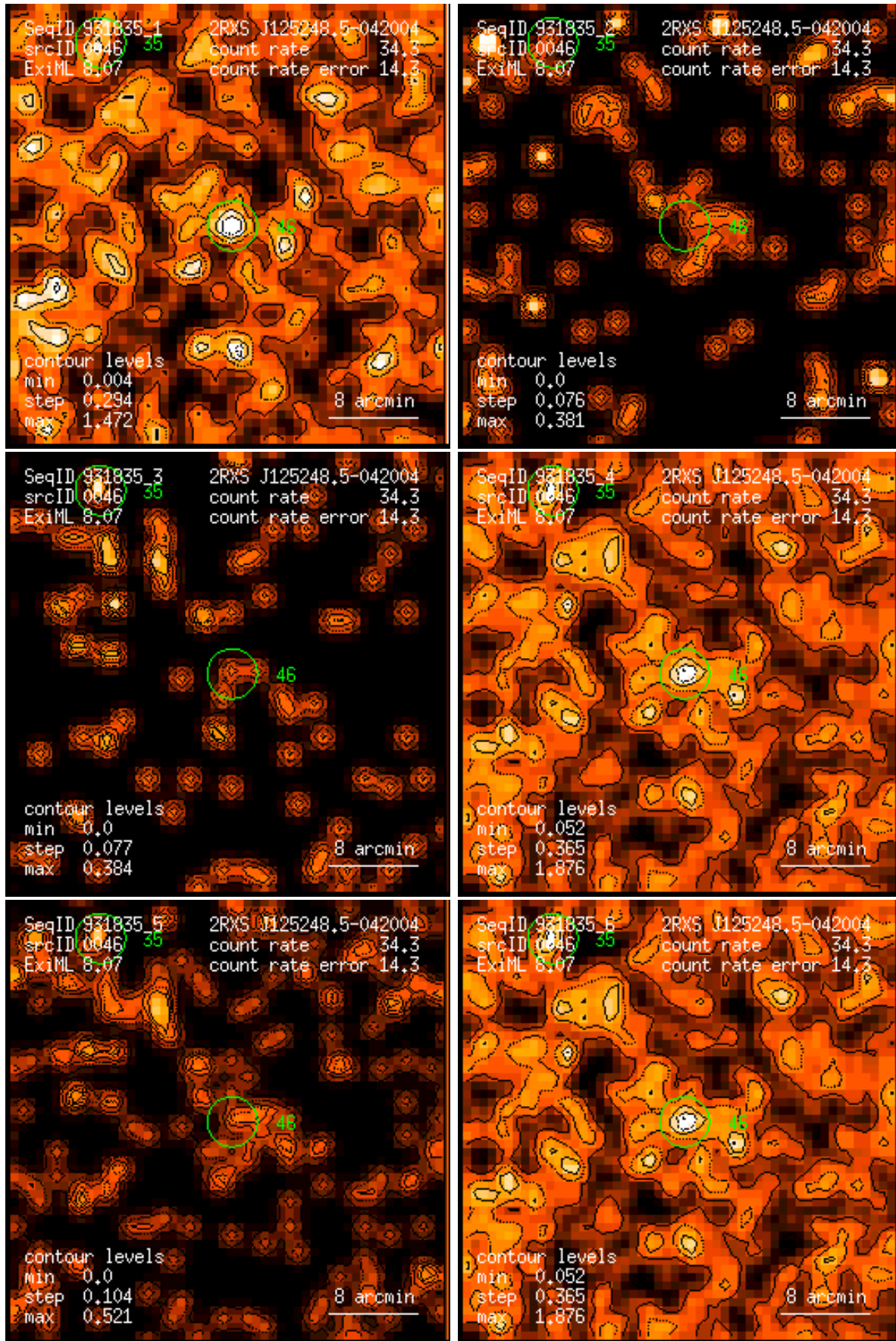
Figure 46: RASS 931835: detection 0046: band rate images, Gaussian filter: (1) PSPC channels 11 – 41, (2) 52 – 90, (3) 91 – 201, (4) 11 – 235, (5) 52 – 201, (6) 11 – 201. Broad band rates in counts/ks. Band rate contour levels in counts/ks/arcmin 2 .
