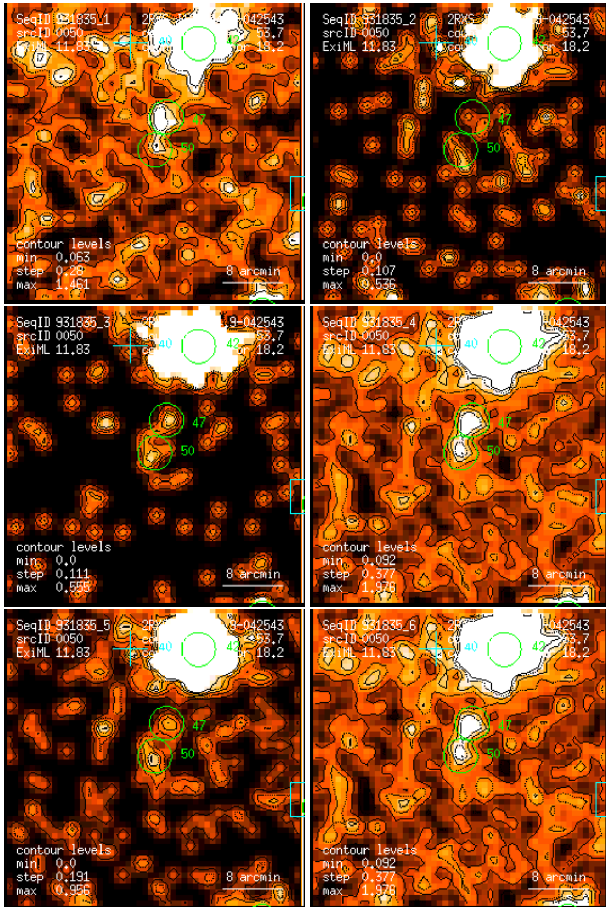
Figure 50: RASS 931835: detection 0050: band rate images, Gaussian filter: (1) PSPC channels 11 – 41, (2) 52 – 90, (3) 91 – 201, (4) 11 – 235, (5) 52 – 201, (6) 11 – 201. Broad band rates in counts/ks. Band rate contour levels in counts/ks/arcmin 2 .
