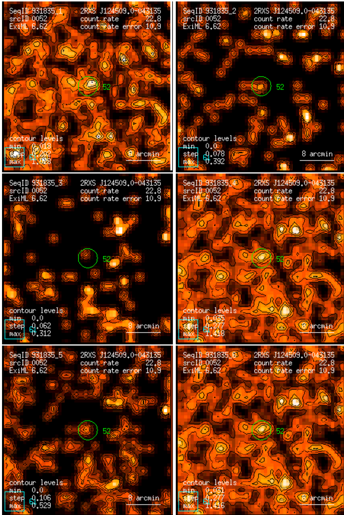
Figure 52: RASS 931835: detection 0052: band rate images, Gaussian filter: (1) PSPC channels 11 – 41, (2) 52 – 90, (3) 91 – 201, (4) 11 – 235, (5) 52 – 201, (6) 11 – 201. Broad band rates in counts/ks. Band rate contour levels in counts/ks/arcmin 2 .
