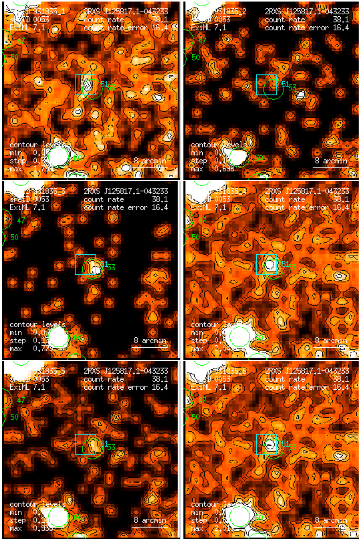
Figure 53: RASS 931835: detection 0053: band rate images, Gaussian filter: (1) PSPC channels 11 – 41, (2) 52 – 90, (3) 91 – 201, (4) 11 – 235, (5) 52 – 201, (6) 11 – 201. Broad band rates in counts/ks. Band rate contour levels in counts/ks/arcmin 2 .
