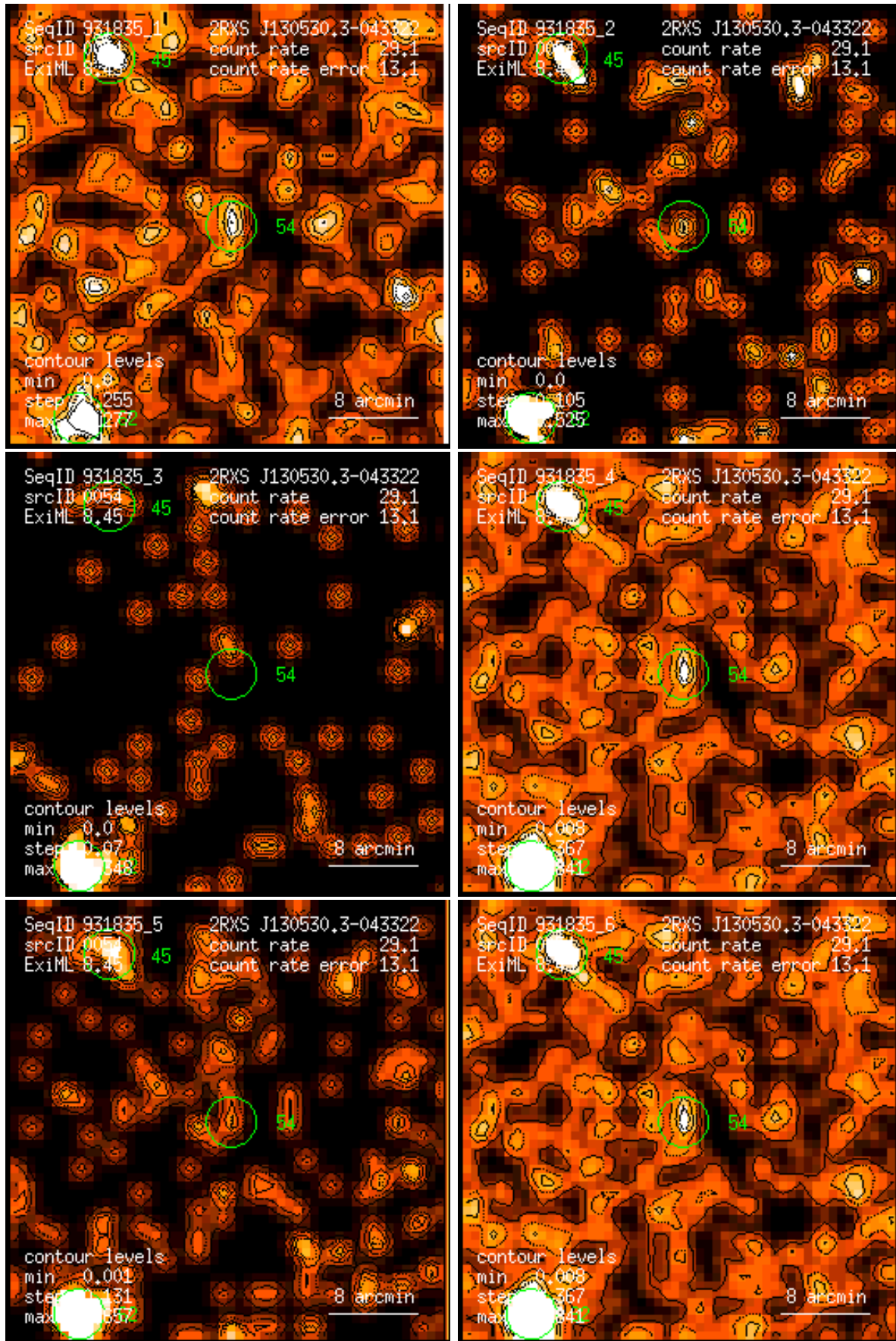
Figure 54: RASS 931835: detection 0054: band rate images, Gaussian filter: (1) PSPC channels 11 – 41, (2) 52 – 90, (3) 91 – 201, (4) 11 – 235, (5) 52 – 201, (6) 11 – 201. Broad band rates in counts/ks. Band rate contour levels in counts/ks/arcmin 2 .
