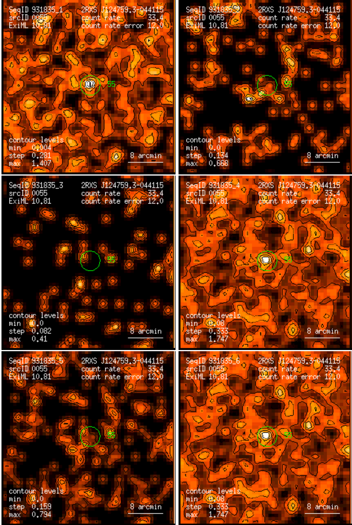
Figure 55: RASS 931835: detection 0055: band rate images, Gaussian filter: (1) PSPC channels 11 – 41, (2) 52 – 90, (3) 91 – 201, (4) 11 – 235, (5) 52 – 201, (6) 11 – 201. Broad band rates in counts/ks. Band rate contour levels in counts/ks/arcmin 2 .
