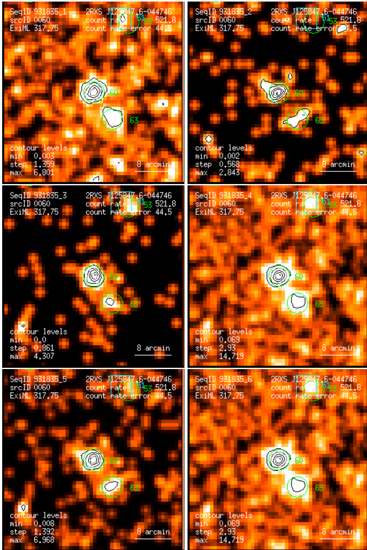
Figure 60: RASS 931835: detection 0060: band rate images, Gaussian filter: (1) PSPC channels 11 – 41, (2) 52 – 90, (3) 91 – 201, (4) 11 – 235, (5) 52 – 201, (6) 11 – 201. Broad band rates in counts/ks. Band rate contour levels in counts/ks/arcmin 2 .
