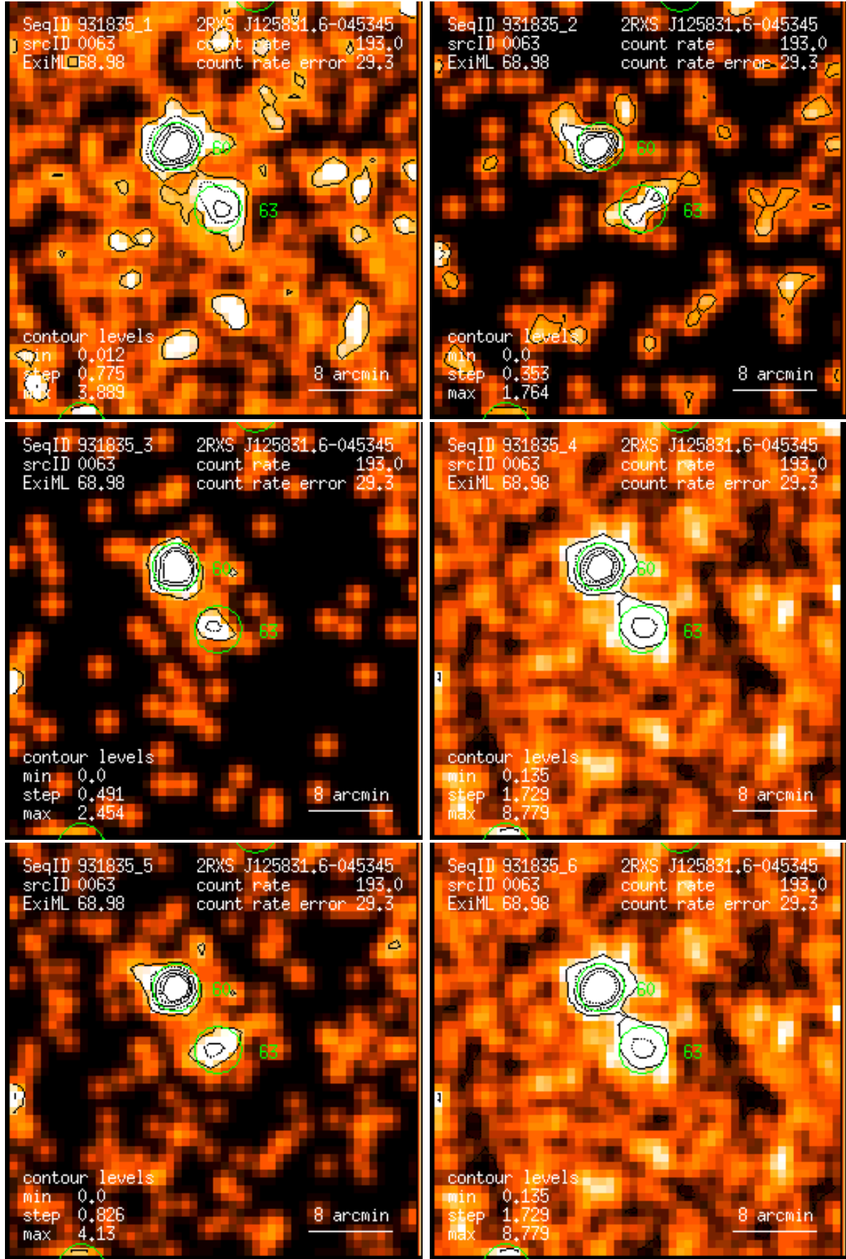
Figure 63: RASS 931835: detection 0063: band rate images, Gaussian filter: (1) PSPC channels 11 – 41, (2) 52 – 90, (3) 91 – 201, (4) 11 – 235, (5) 52 – 201, (6) 11 – 201. Broad band rates in counts/ks. Band rate contour levels in counts/ks/arcmin 2 .
