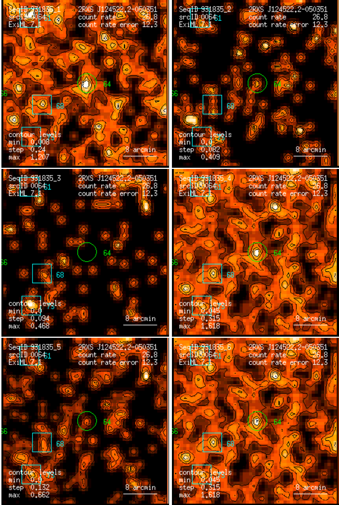
Figure 64: RASS 931835: detection 0064: band rate images, Gaussian filter: (1) PSPC channels 11 – 41, (2) 52 – 90, (3) 91 – 201, (4) 11 – 235, (5) 52 – 201, (6) 11 – 201. Broad band rates in counts/ks. Band rate contour levels in counts/ks/arcmin 2 .
