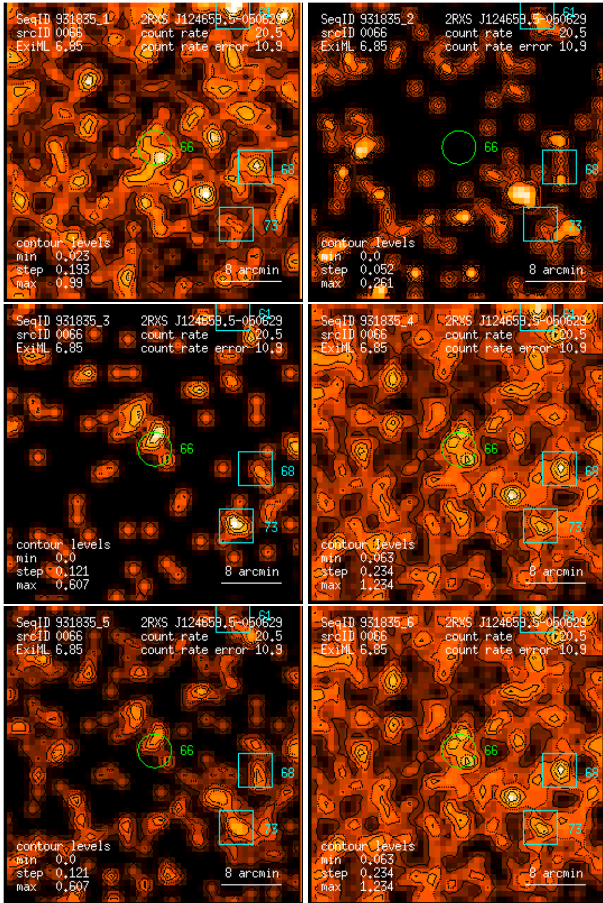
Figure 66: RASS 931835: detection 0066: band rate images, Gaussian filter: (1) PSPC channels 11 – 41, (2) 52 – 90, (3) 91 – 201, (4) 11 – 235, (5) 52 – 201, (6) 11 – 201. Broad band rates in counts/ks. Band rate contour levels in counts/ks/arcmin 2 .
