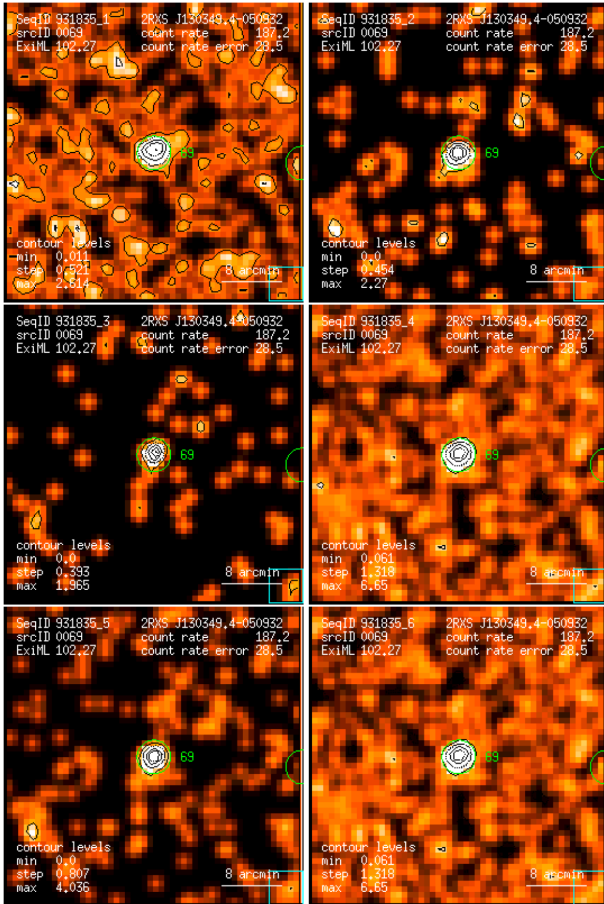
Figure 69: RASS 931835: detection 0069: band rate images, Gaussian filter: (1) PSPC channels 11 – 41, (2) 52 – 90, (3) 91 – 201, (4) 11 – 235, (5) 52 – 201, (6) 11 – 201. Broad band rates in counts/ks. Band rate contour levels in counts/ks/arcmin 2 .
