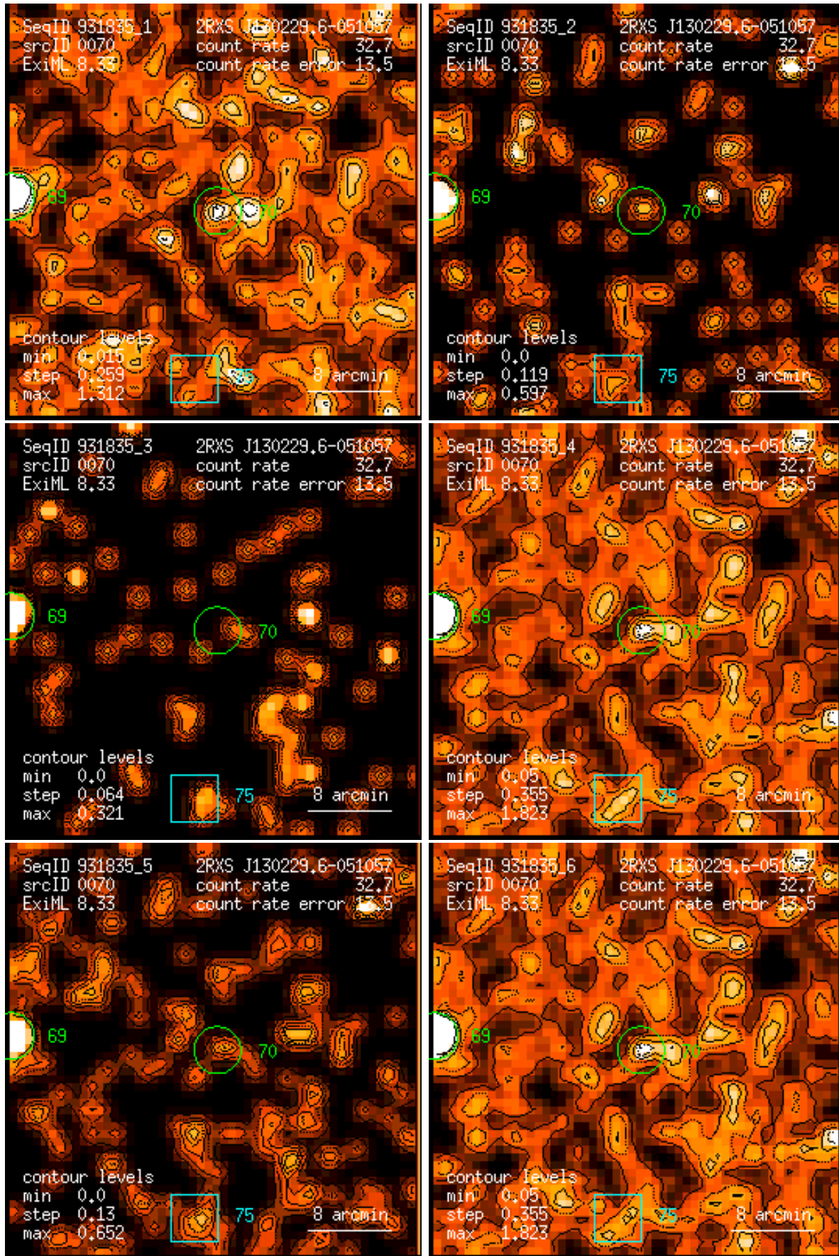
Figure 70: RASS 931835: detection 0070: band rate images, Gaussian filter: (1) PSPC channels 11 – 41, (2) 52 – 90, (3) 91 – 201, (4) 11 – 235, (5) 52 – 201, (6) 11 – 201. Broad band rates in counts/ks. Band rate contour levels in counts/ks/arcmin 2 .
