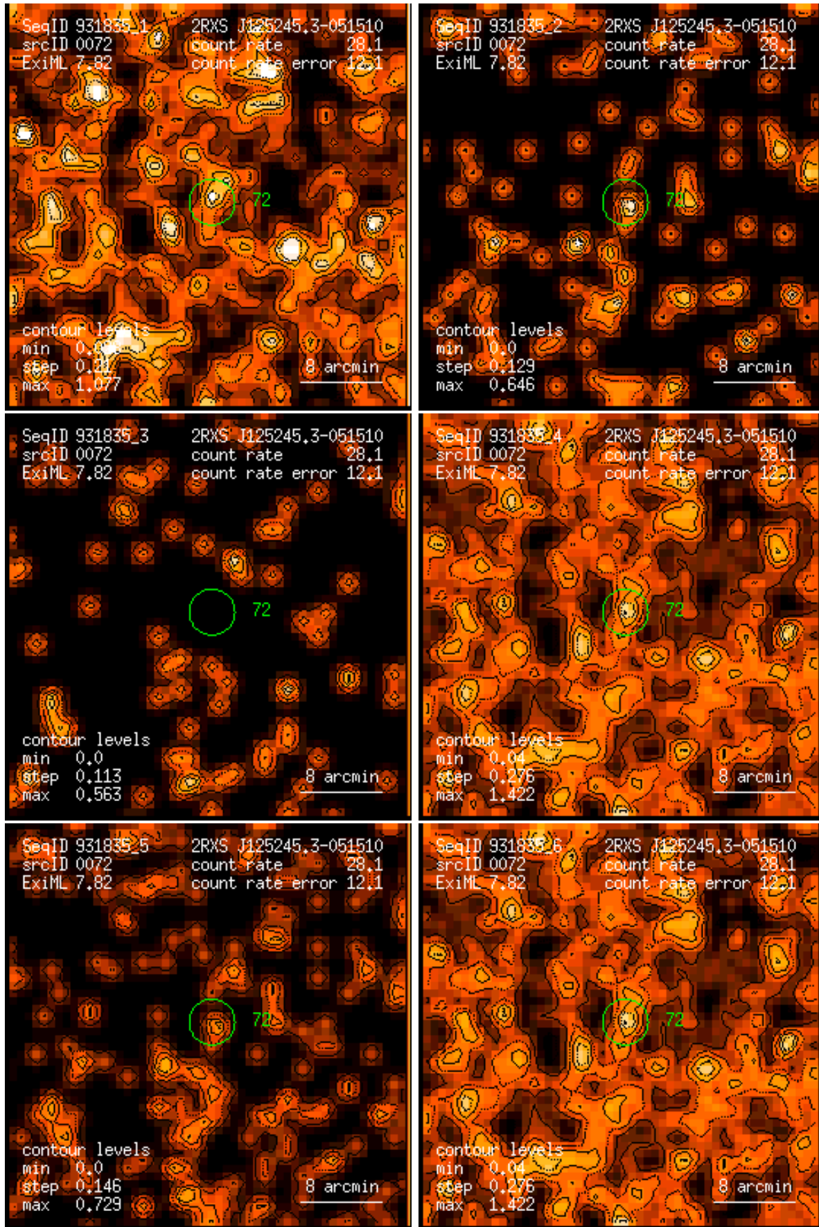
Figure 72: RASS 931835: detection 0072: band rate images, Gaussian filter: (1) PSPC channels 11 – 41, (2) 52 – 90, (3) 91 – 201, (4) 11 – 235, (5) 52 – 201, (6) 11 – 201. Broad band rates in counts/ks. Band rate contour levels in counts/ks/arcmin 2 .
